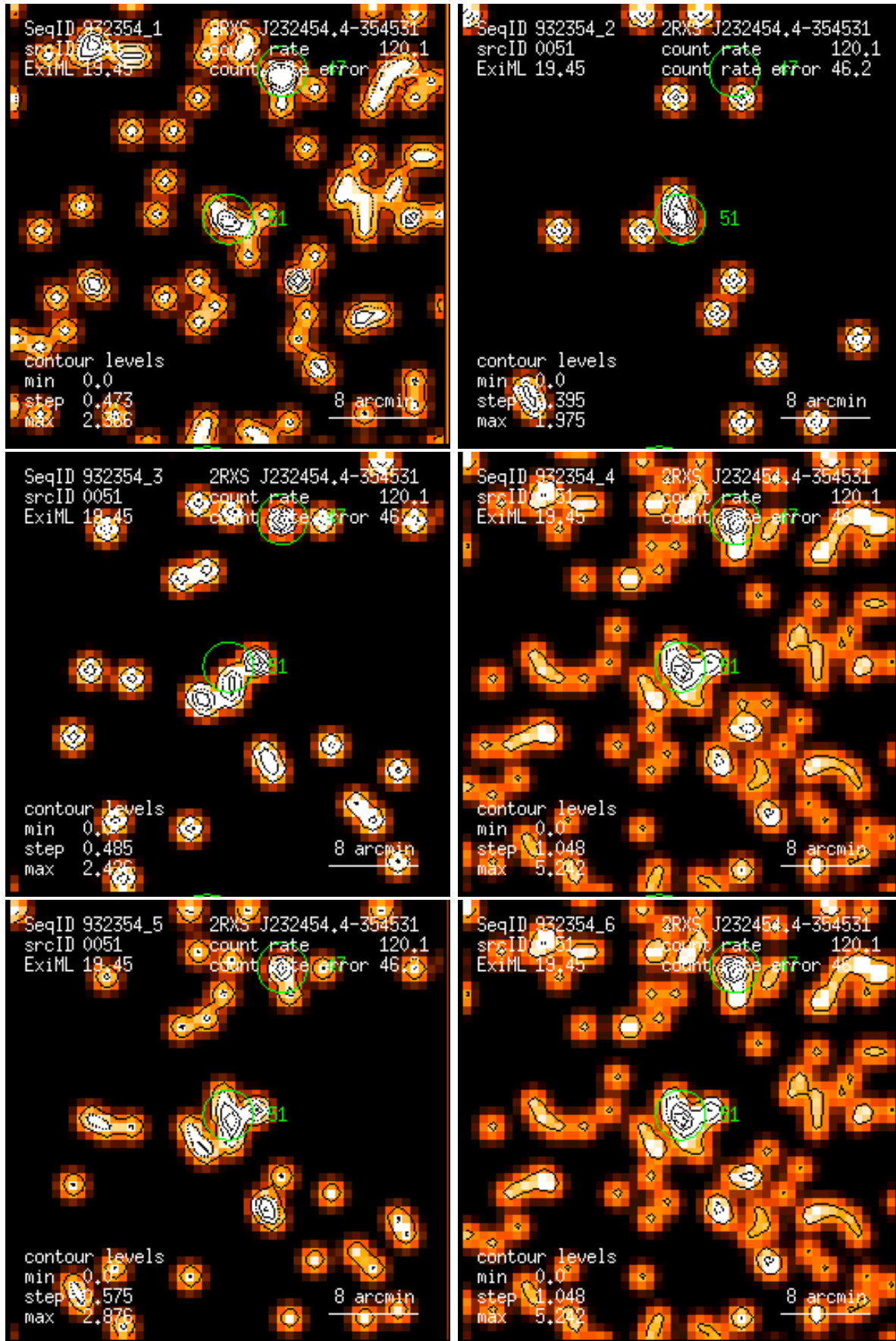
Figure 51: RASS 932354: detection 0051: band rate images, Gaussian filter: (1) PSPC channels 11 – 41, (2) 52 – 90, (3) 91 – 201, (4) 11 – 235, (5) 52 – 201, (6) 11 – 201. Broad band rates in counts/ks. Band rate contour levels in counts/ks/arcmin 2 .
