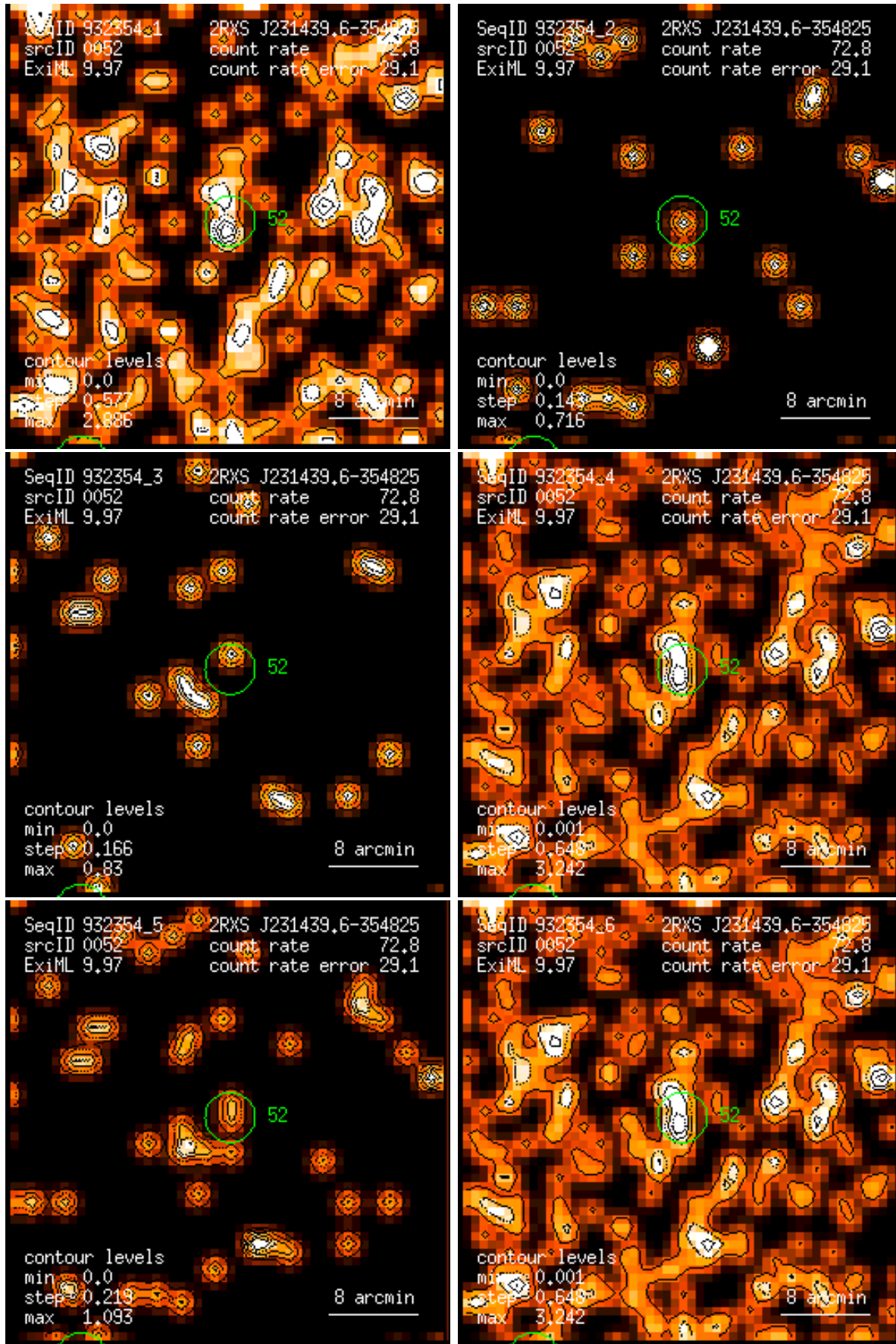
Figure 52: RASS 932354: detection 0052: band rate images, Gaussian filter: (1) PSPC channels 11 – 41, (2) 52 – 90, (3) 91 – 201, (4) 11 – 235, (5) 52 – 201, (6) 11 – 201. Broad band rates in counts/ks. Band rate contour levels in counts/ks/arcmin 2 .
