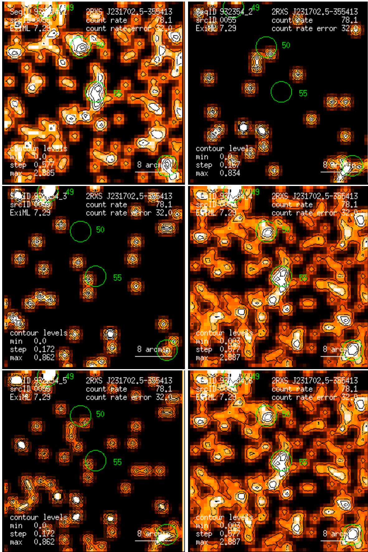
Figure 55: RASS 932354: detection 0055: band rate images, Gaussian filter: (1) PSPC channels 11 – 41, (2) 52 – 90, (3) 91 – 201, (4) 11 – 235, (5) 52 – 201, (6) 11 – 201. Broad band rates in counts/ks. Band rate contour levels in counts/ks/arcmin 2 .
