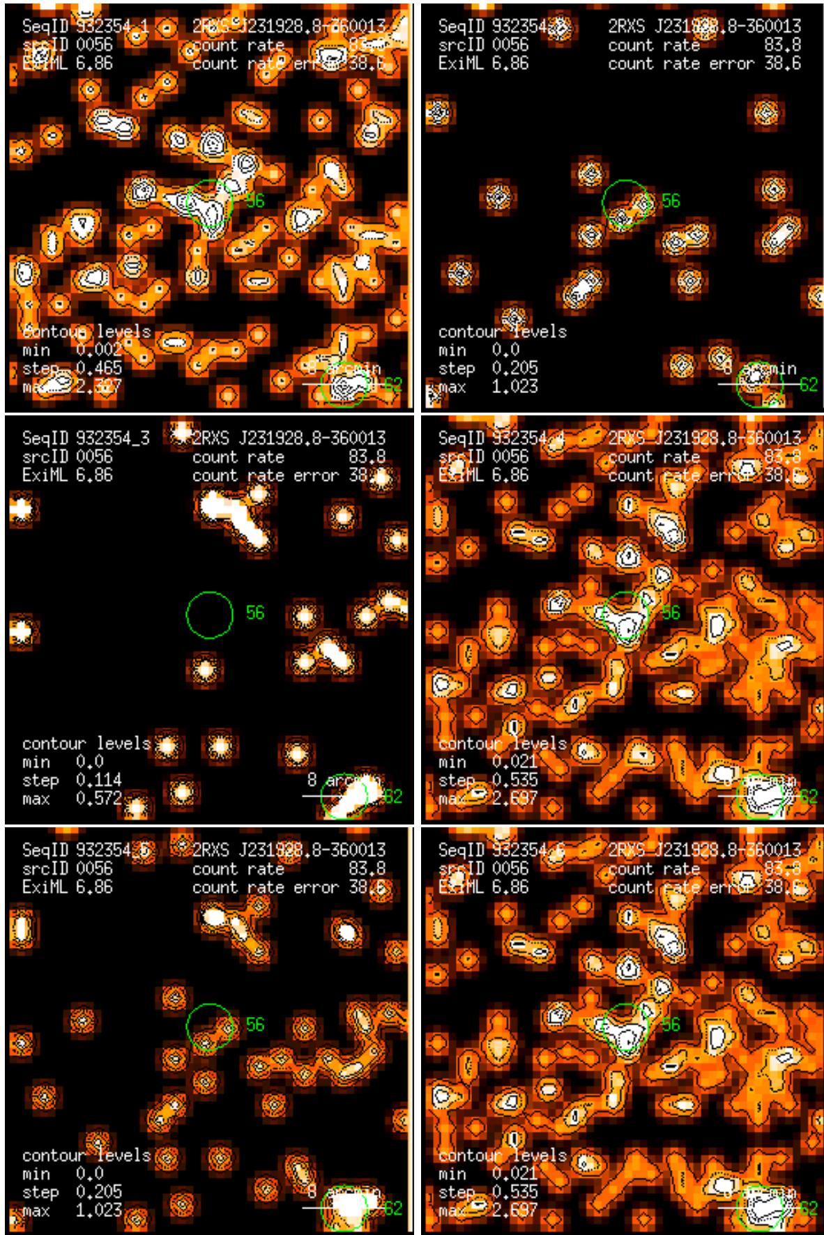
Figure 56: RASS 932354: detection 0056: band rate images, Gaussian filter: (1) PSPC channels 11 – 41, (2) 52 – 90, (3) 91 – 201, (4) 11 – 235, (5) 52 – 201, (6) 11 – 201. Broad band rates in counts/ks. Band rate contour levels in counts/ks/arcmin 2 .
