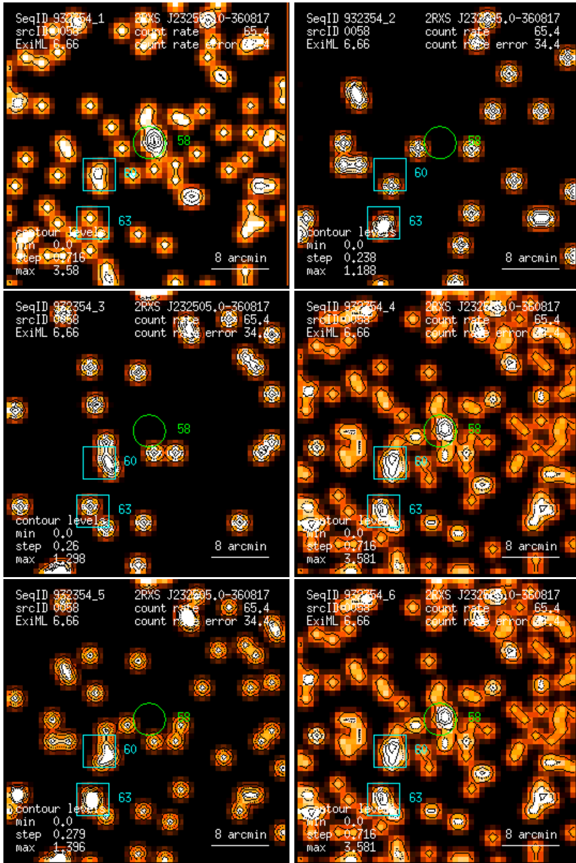
Figure 58: RASS 932354: detection 0058: band rate images, Gaussian filter: (1) PSPC channels 11 – 41, (2) 52 – 90, (3) 91 – 201, (4) 11 – 235, (5) 52 – 201, (6) 11 – 201. Broad band rates in counts/ks. Band rate contour levels in counts/ks/arcmin 2 .
