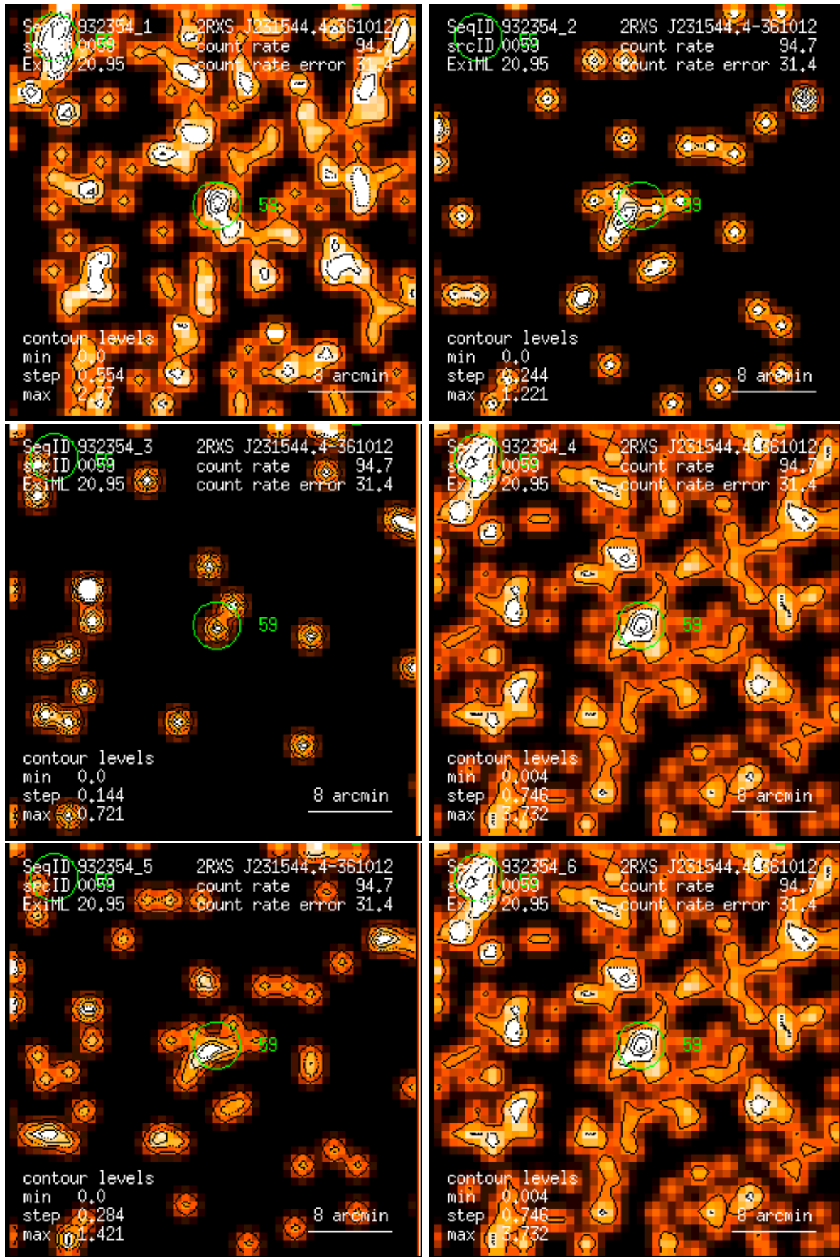
Figure 59: RASS 932354: detection 0059: band rate images, Gaussian filter: (1) PSPC channels 11 – 41, (2) 52 – 90, (3) 91 – 201, (4) 11 – 235, (5) 52 – 201, (6) 11 – 201. Broad band rates in counts/ks. Band rate contour levels in counts/ks/arcmin 2 .
