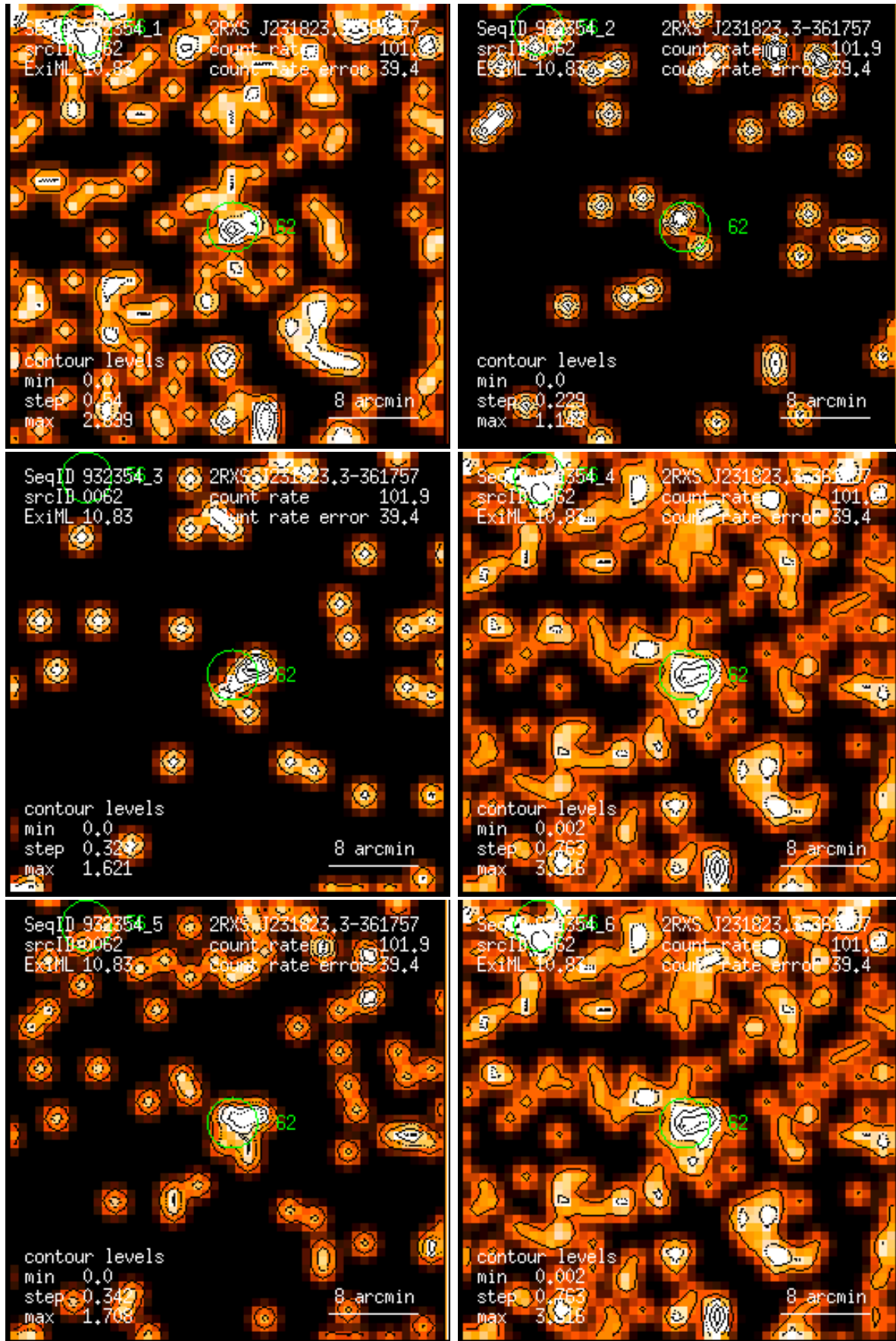
Figure 62: RASS 932354: detection 0062: band rate images, Gaussian filter: (1) PSPC channels 11 – 41, (2) 52 – 90, (3) 91 – 201, (4) 11 – 235, (5) 52 – 201, (6) 11 – 201. Broad band rates in counts/ks. Band rate contour levels in counts/ks/arcmin 2 .
