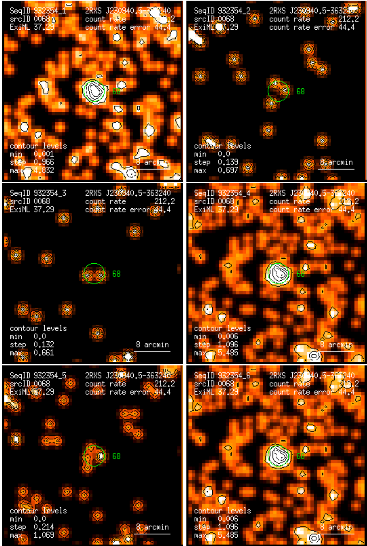
Figure 68: RASS 932354: detection 0068: band rate images, Gaussian filter: (1) PSPC channels 11 – 41, (2) 52 – 90, (3) 91 – 201, (4) 11 – 235, (5) 52 – 201, (6) 11 – 201. Broad band rates in counts/ks. Band rate contour levels in counts/ks/arcmin 2 .
