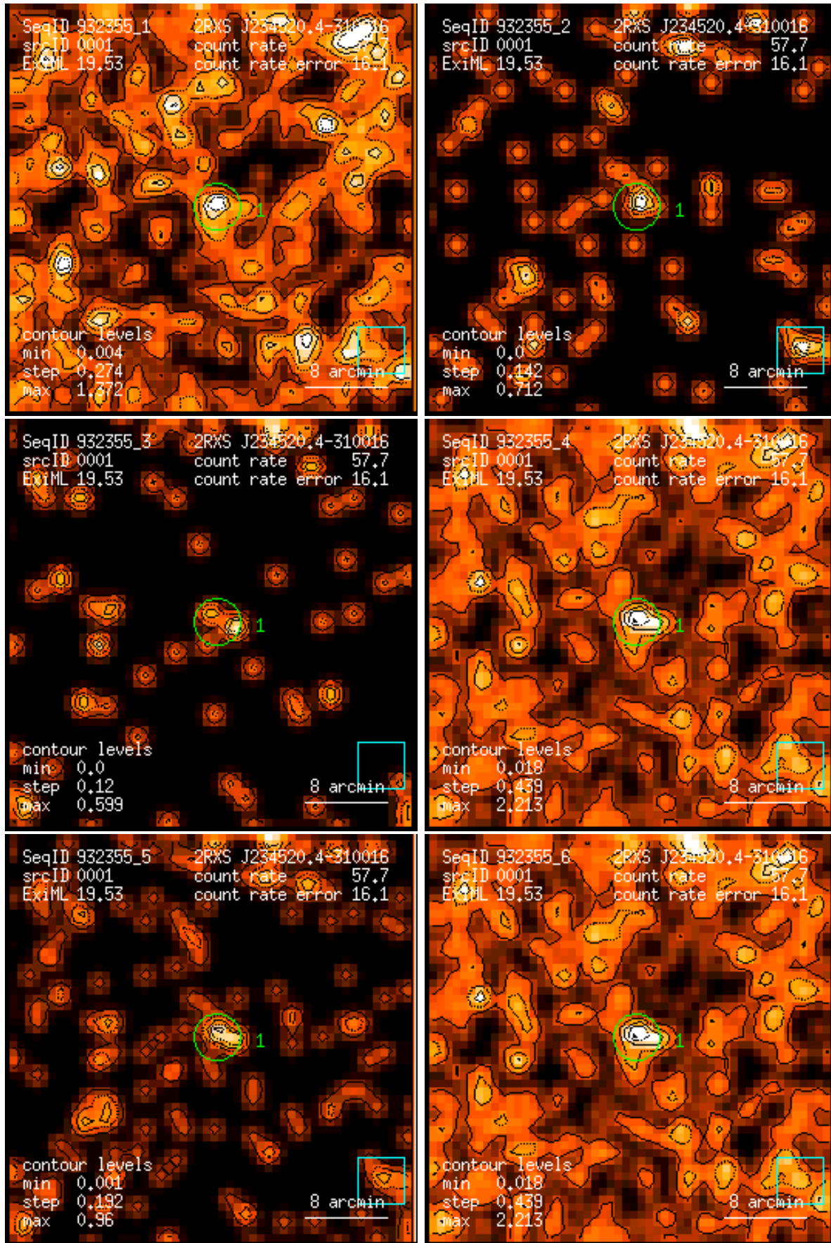
Figure 1: RASS 932355: detection 0001: band rate images, Gaussian filter: (1) PSPC channels 11 – 41, (2) 52 – 90, (3) 91 – 201, (4) 11 – 235, (5) 52 – 201, (6) 11 – 201. Broad band rates in counts/ks. Band rate contour levels in counts/ks/arcmin 2 .
