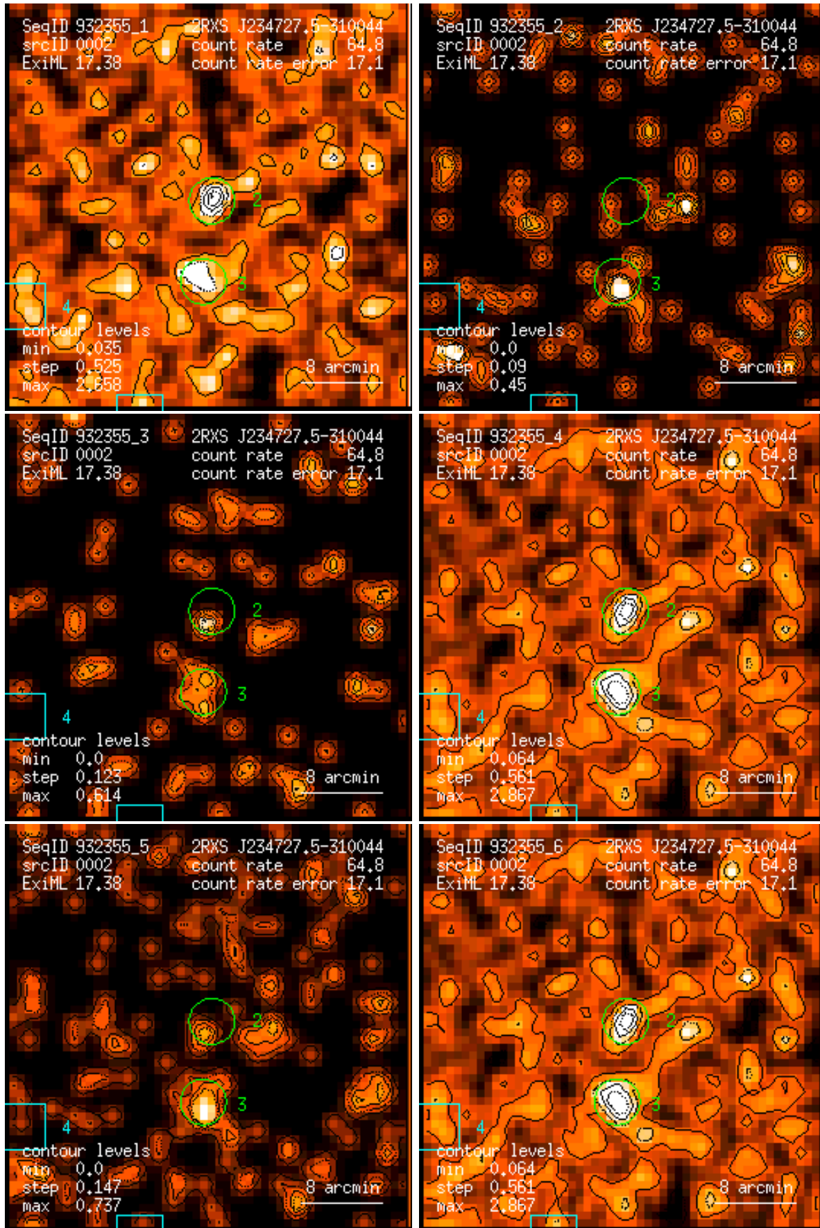
Figure 2: RASS 932355: detection 0002: band rate images, Gaussian filter: (1) PSPC channels 11 – 41, (2) 52 – 90, (3) 91 – 201, (4) 11 – 235, (5) 52 – 201, (6) 11 – 201. Broad band rates in counts/ks. Band rate contour levels in counts/ks/arcmin 2 .
