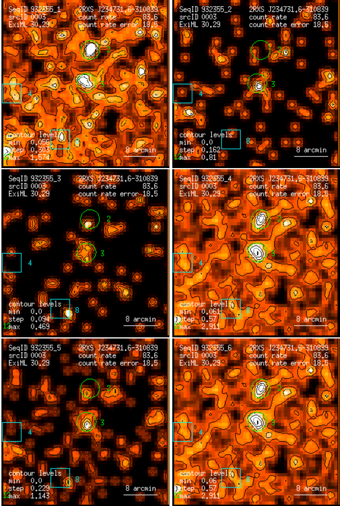
Figure 3: RASS 932355: detection 0003: band rate images, Gaussian filter: (1) PSPC channels 11 – 41, (2) 52 – 90, (3) 91 – 201, (4) 11 – 235, (5) 52 – 201, (6) 11 – 201. Broad band rates in counts/ks. Band rate contour levels in counts/ks/arcmin 2 .
