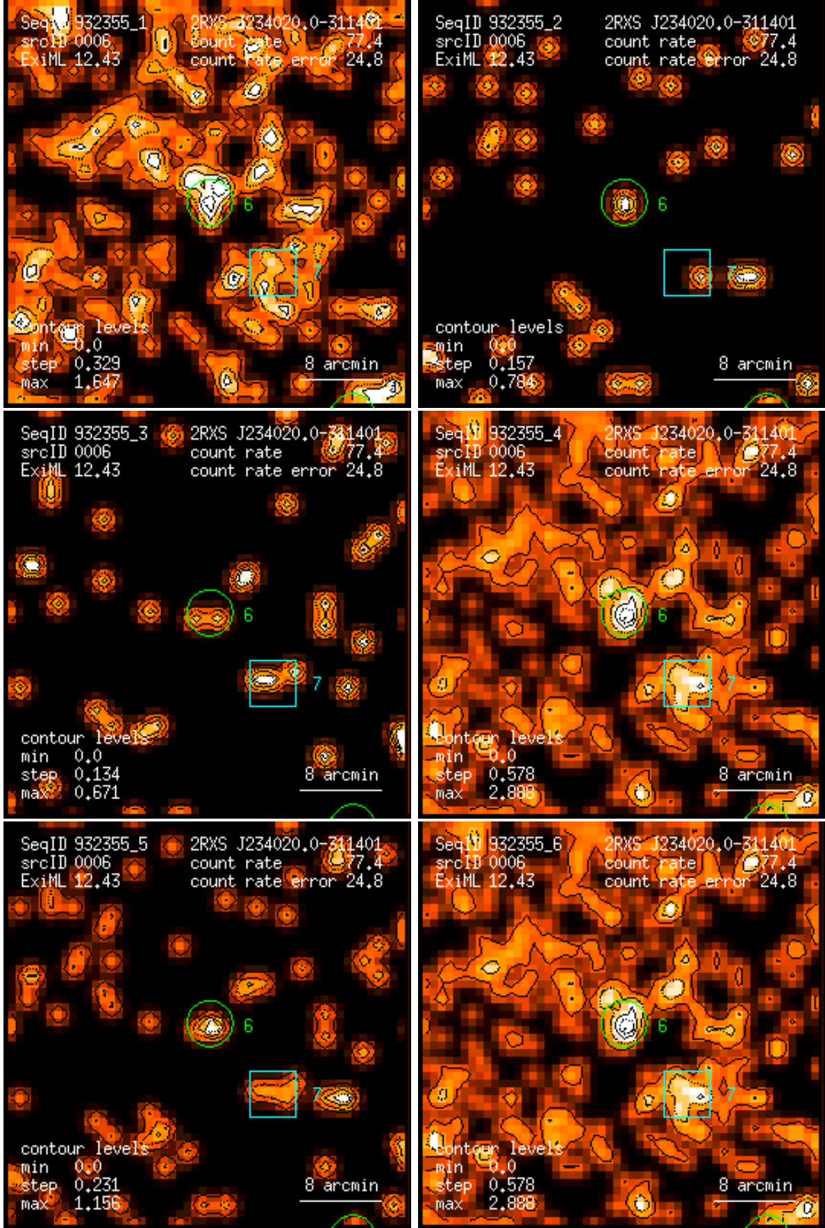
Figure 6: RASS 932355: detection 0006: band rate images, Gaussian filter: (1) PSPC channels 11 – 41, (2) 52 – 90, (3) 91 – 201, (4) 11 – 235, (5) 52 – 201, (6) 11 – 201. Broad band rates in counts/ks. Band rate contour levels in counts/ks/arcmin 2 .
