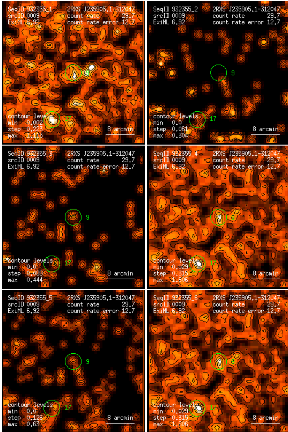
Figure 9: RASS 932355: detection 0009: band rate images, Gaussian filter: (1) PSPC channels 11 – 41, (2) 52 – 90, (3) 91 – 201, (4) 11 – 235, (5) 52 – 201, (6) 11 – 201. Broad band rates in counts/ks. Band rate contour levels in counts/ks/arcmin 2 .
