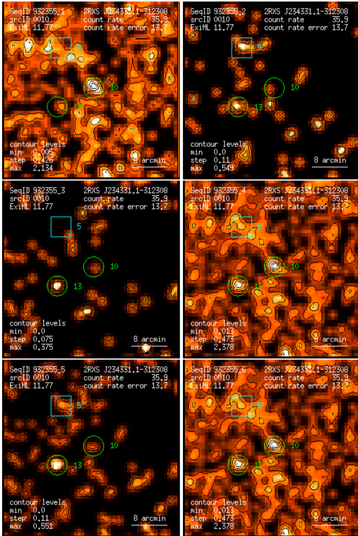
Figure 10: RASS 932355: detection 0010: band rate images, Gaussian filter: (1) PSPC channels 11 – 41, (2) 52 – 90, (3) 91 – 201, (4) 11 – 235, (5) 52 – 201, (6) 11 – 201. Broad band rates in counts/ks. Band rate contour levels in counts/ks/arcmin 2 .
