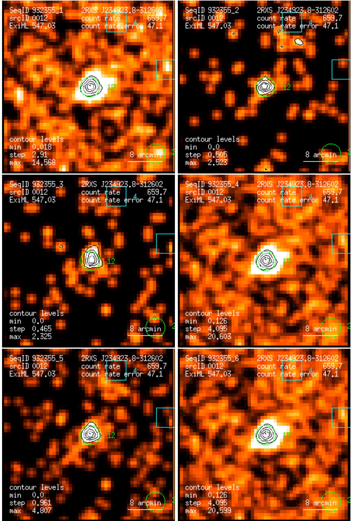
Figure 12: RASS 932355: detection 0012: band rate images, Gaussian filter: (1) PSPC channels 11 – 41, (2) 52 – 90, (3) 91 – 201, (4) 11 – 235, (5) 52 – 201, (6) 11 – 201. Broad band rates in counts/ks. Band rate contour levels in counts/ks/arcmin 2 .
