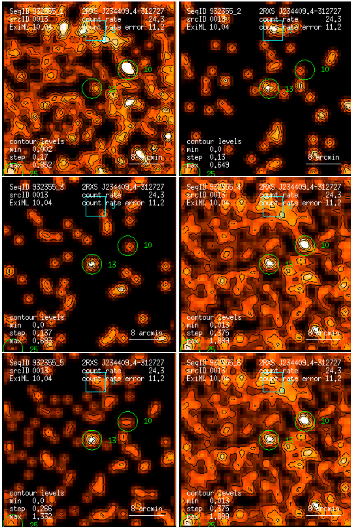
Figure 13: RASS 932355: detection 0013: band rate images, Gaussian filter: (1) PSPC channels 11 – 41, (2) 52 – 90, (3) 91 – 201, (4) 11 – 235, (5) 52 – 201, (6) 11 – 201. Broad band rates in counts/ks. Band rate contour levels in counts/ks/arcmin 2 .
