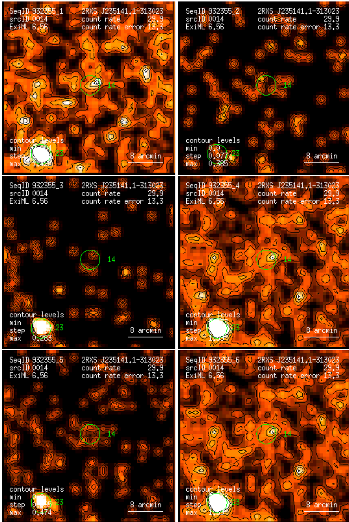
Figure 14: RASS 932355: detection 0014: band rate images, Gaussian filter: (1) PSPC channels 11 – 41, (2) 52 – 90, (3) 91 – 201, (4) 11 – 235, (5) 52 – 201, (6) 11 – 201. Broad band rates in counts/ks. Band rate contour levels in counts/ks/arcmin 2 .
