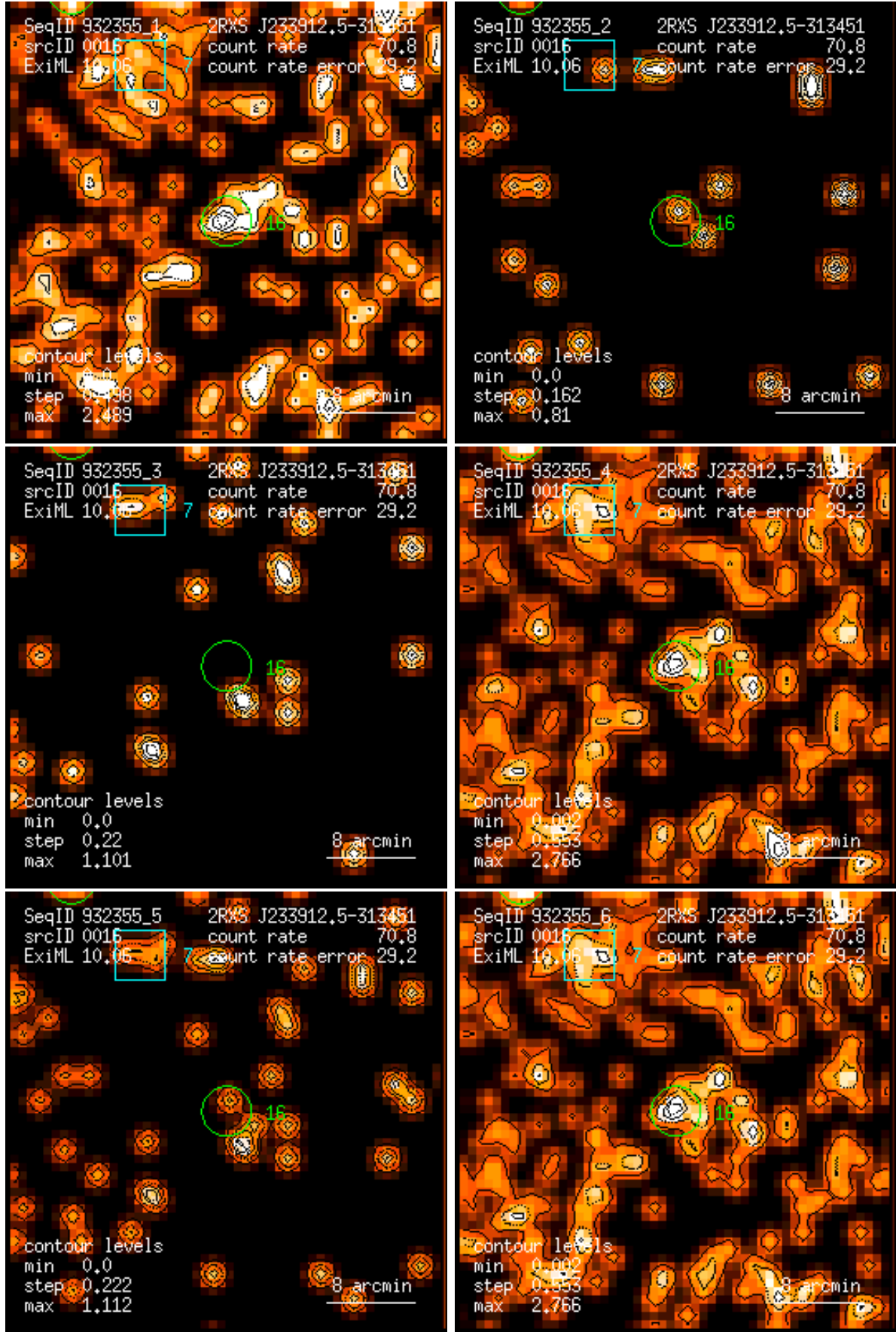
Figure 16: RASS 932355: detection 0016: band rate images, Gaussian filter: (1) PSPC channels 11 – 41, (2) 52 – 90, (3) 91 – 201, (4) 11 – 235, (5) 52 – 201, (6) 11 – 201. Broad band rates in counts/ks. Band rate contour levels in counts/ks/arcmin 2 .
