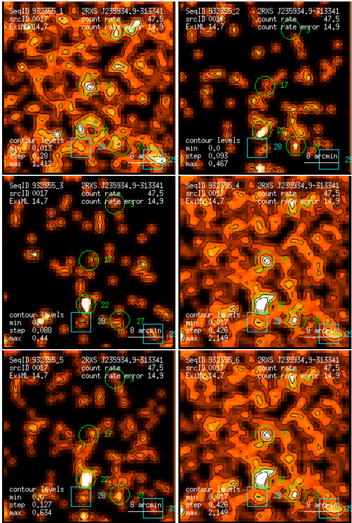
Figure 17: RASS 932355: detection 0017: band rate images, Gaussian filter: (1) PSPC channels 11 – 41, (2) 52 – 90, (3) 91 – 201, (4) 11 – 235, (5) 52 – 201, (6) 11 – 201. Broad band rates in counts/ks. Band rate contour levels in counts/ks/arcmin 2 .
