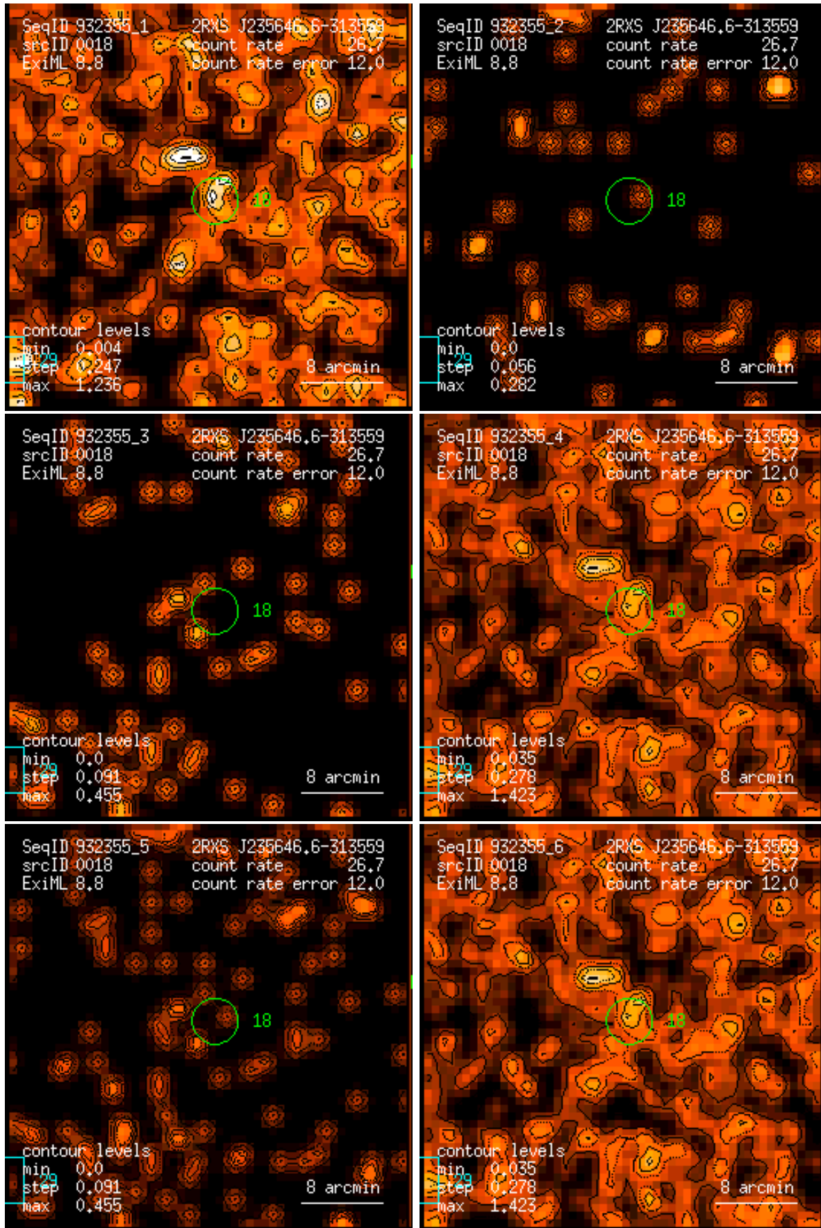
Figure 18: RASS 932355: detection 0018: band rate images, Gaussian filter: (1) PSPC channels 11 – 41, (2) 52 – 90, (3) 91 – 201, (4) 11 – 235, (5) 52 – 201, (6) 11 – 201. Broad band rates in counts/ks. Band rate contour levels in counts/ks/arcmin 2 .
