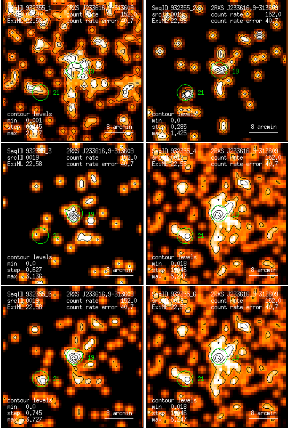
Figure 19: RASS 932355: detection 0019: band rate images, Gaussian filter: (1) PSPC channels 11 – 41, (2) 52 – 90, (3) 91 – 201, (4) 11 – 235, (5) 52 – 201, (6) 11 – 201. Broad band rates in counts/ks. Band rate contour levels in counts/ks/arcmin 2 .
