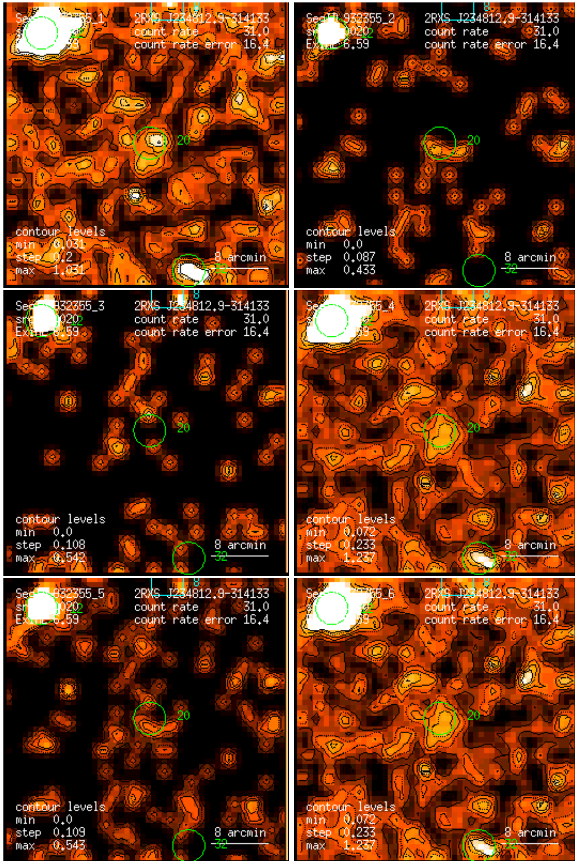
Figure 20: RASS 932355: detection 0020: band rate images, Gaussian filter: (1) PSPC channels 11 – 41, (2) 52 – 90, (3) 91 – 201, (4) 11 – 235, (5) 52 – 201, (6) 11 – 201. Broad band rates in counts/ks. Band rate contour levels in counts/ks/arcmin 2 .
