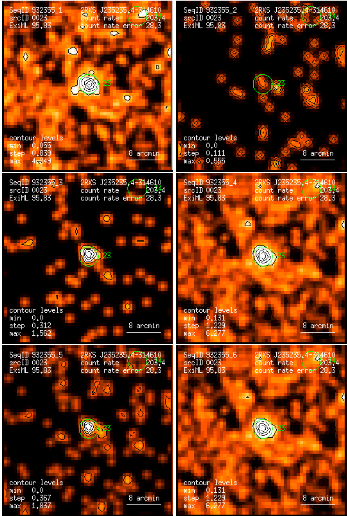
Figure 23: RASS 932355: detection 0023: band rate images, Gaussian filter: (1) PSPC channels 11 – 41, (2) 52 – 90, (3) 91 – 201, (4) 11 – 235, (5) 52 – 201, (6) 11 – 201. Broad band rates in counts/ks. Band rate contour levels in counts/ks/arcmin 2 .
