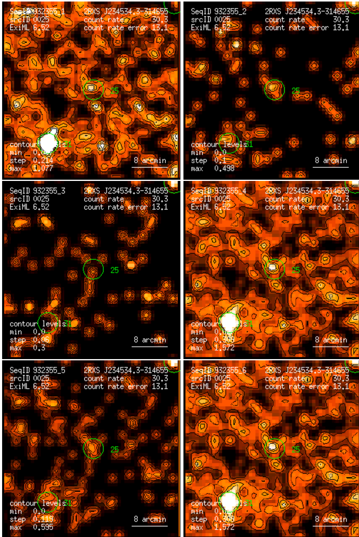
Figure 25: RASS 932355: detection 0025: band rate images, Gaussian filter: (1) PSPC channels 11 – 41, (2) 52 – 90, (3) 91 – 201, (4) 11 – 235, (5) 52 – 201, (6) 11 – 201. Broad band rates in counts/ks. Band rate contour levels in counts/ks/arcmin 2 .
