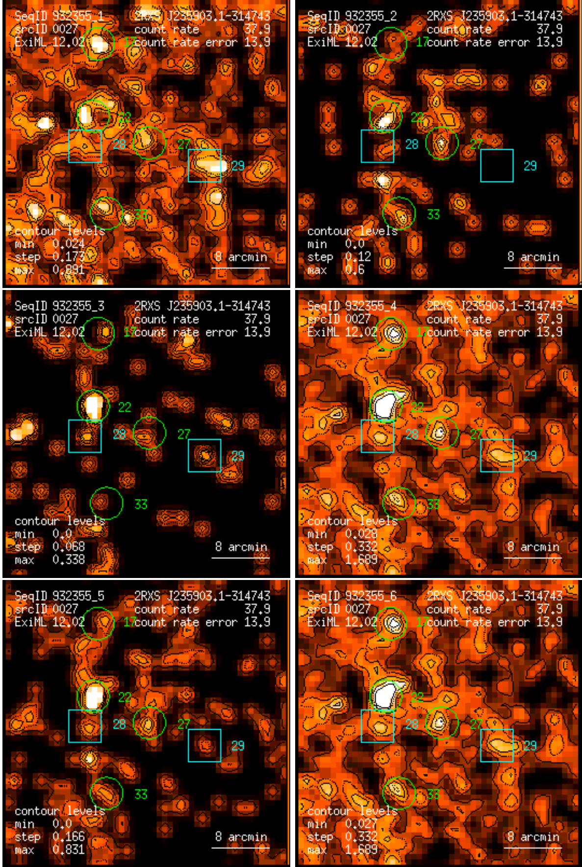
Figure 27: RASS 932355: detection 0027: band rate images, Gaussian filter: (1) PSPC channels 11 – 41, (2) 52 – 90, (3) 91 – 201, (4) 11 – 235, (5) 52 – 201, (6) 11 – 201. Broad band rates in counts/ks. Band rate contour levels in counts/ks/arcmin 2 .
