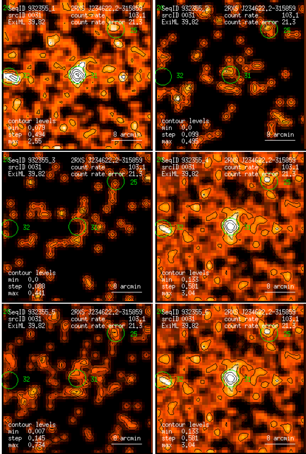
Figure 31: RASS 932355: detection 0031: band rate images, Gaussian filter: (1) PSPC channels 11 – 41, (2) 52 – 90, (3) 91 – 201, (4) 11 – 235, (5) 52 – 201, (6) 11 – 201. Broad band rates in counts/ks. Band rate contour levels in counts/ks/arcmin 2 .
