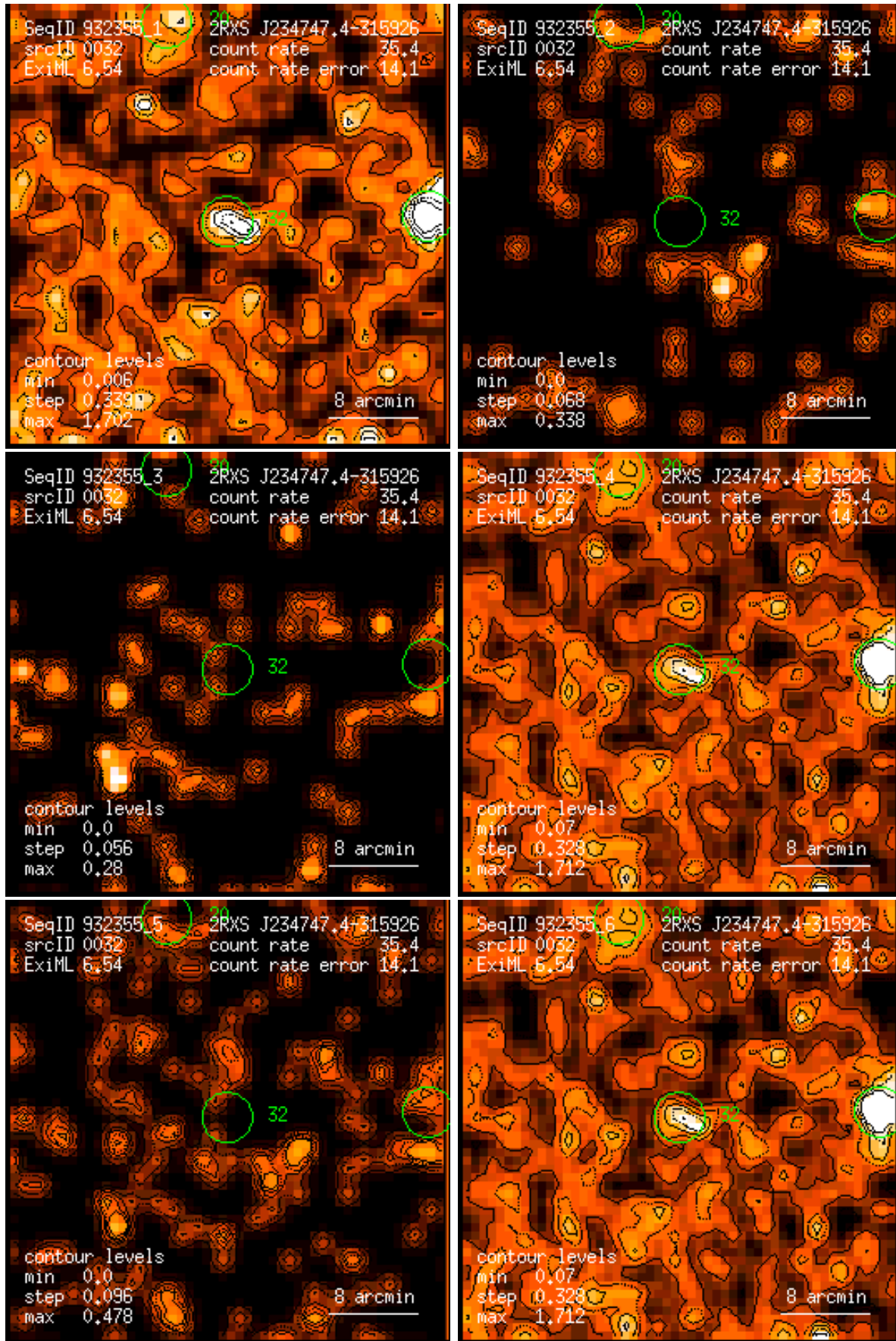
Figure 32: RASS 932355: detection 0032: band rate images, Gaussian filter: (1) PSPC channels 11 – 41, (2) 52 – 90, (3) 91 – 201, (4) 11 – 235, (5) 52 – 201, (6) 11 – 201. Broad band rates in counts/ks. Band rate contour levels in counts/ks/arcmin 2 .
