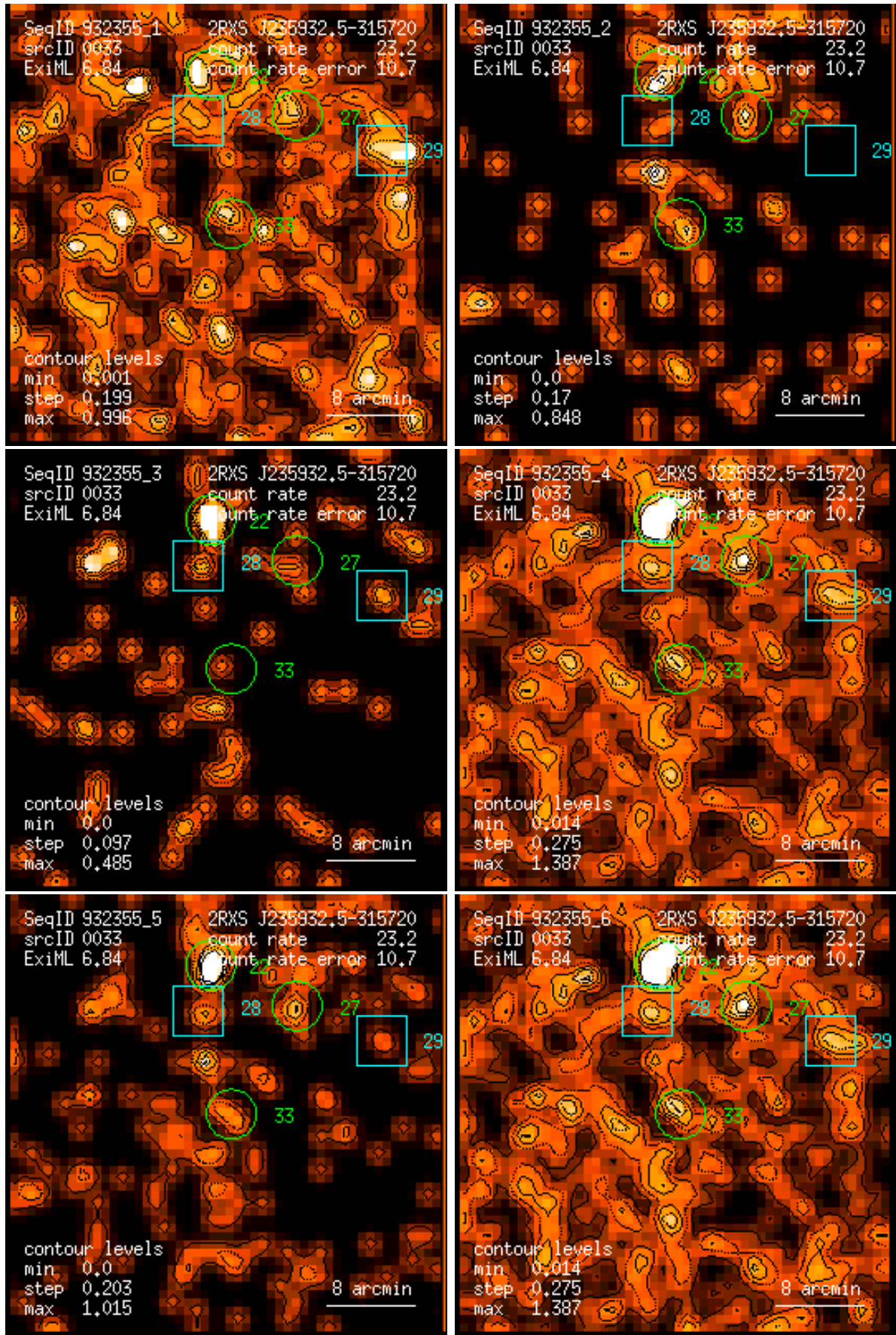
Figure 33: RASS 932355: detection 0033: band rate images, Gaussian filter: (1) PSPC channels 11 – 41, (2) 52 – 90, (3) 91 – 201, (4) 11 – 235, (5) 52 – 201, (6) 11 – 201. Broad band rates in counts/ks. Band rate contour levels in counts/ks/arcmin 2 .
