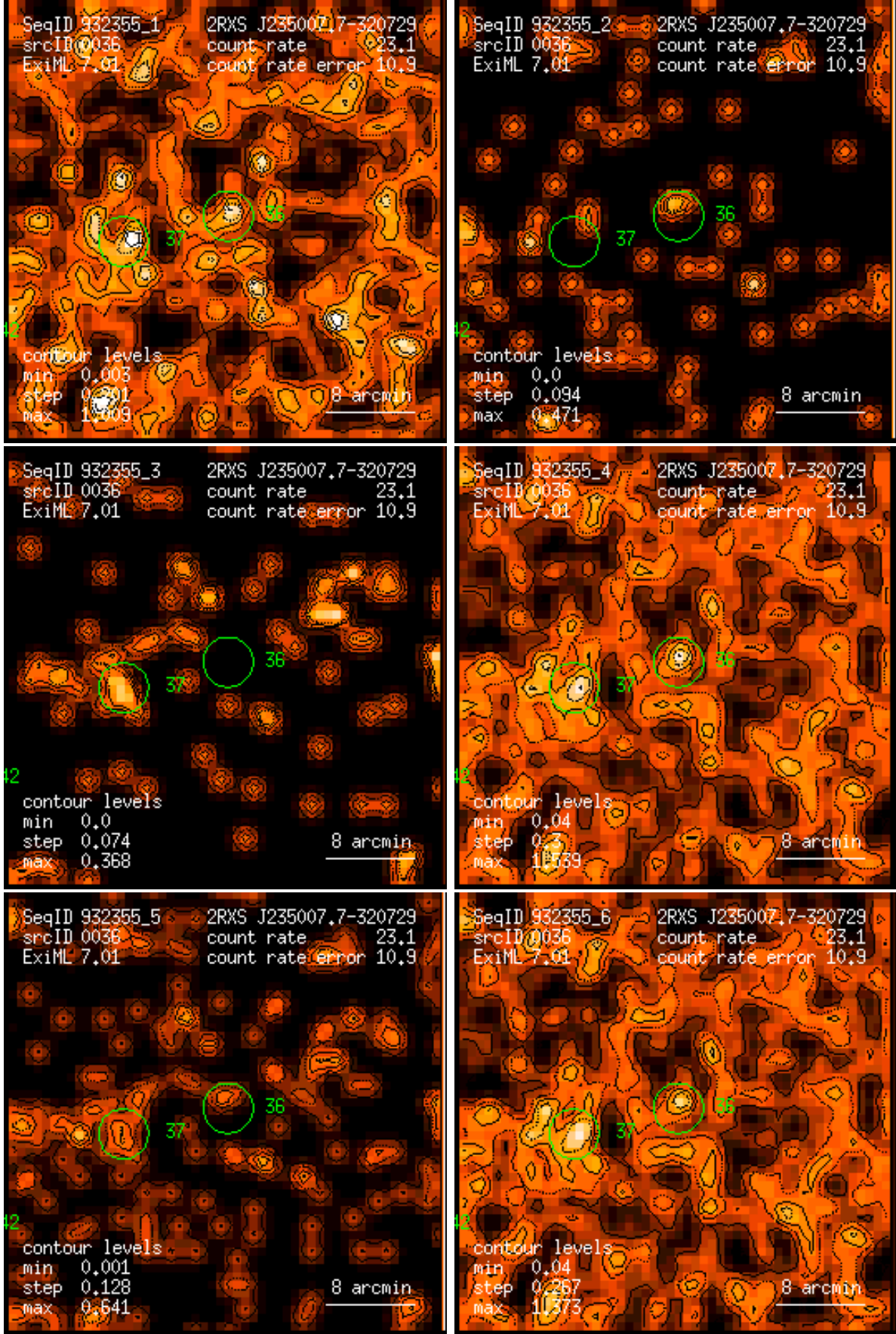
Figure 36: RASS 932355: detection 0036: band rate images, Gaussian filter: (1) PSPC channels 11 – 41, (2) 52 – 90, (3) 91 – 201, (4) 11 – 235, (5) 52 – 201, (6) 11 – 201. Broad band rates in counts/ks. Band rate contour levels in counts/ks/arcmin 2 .
