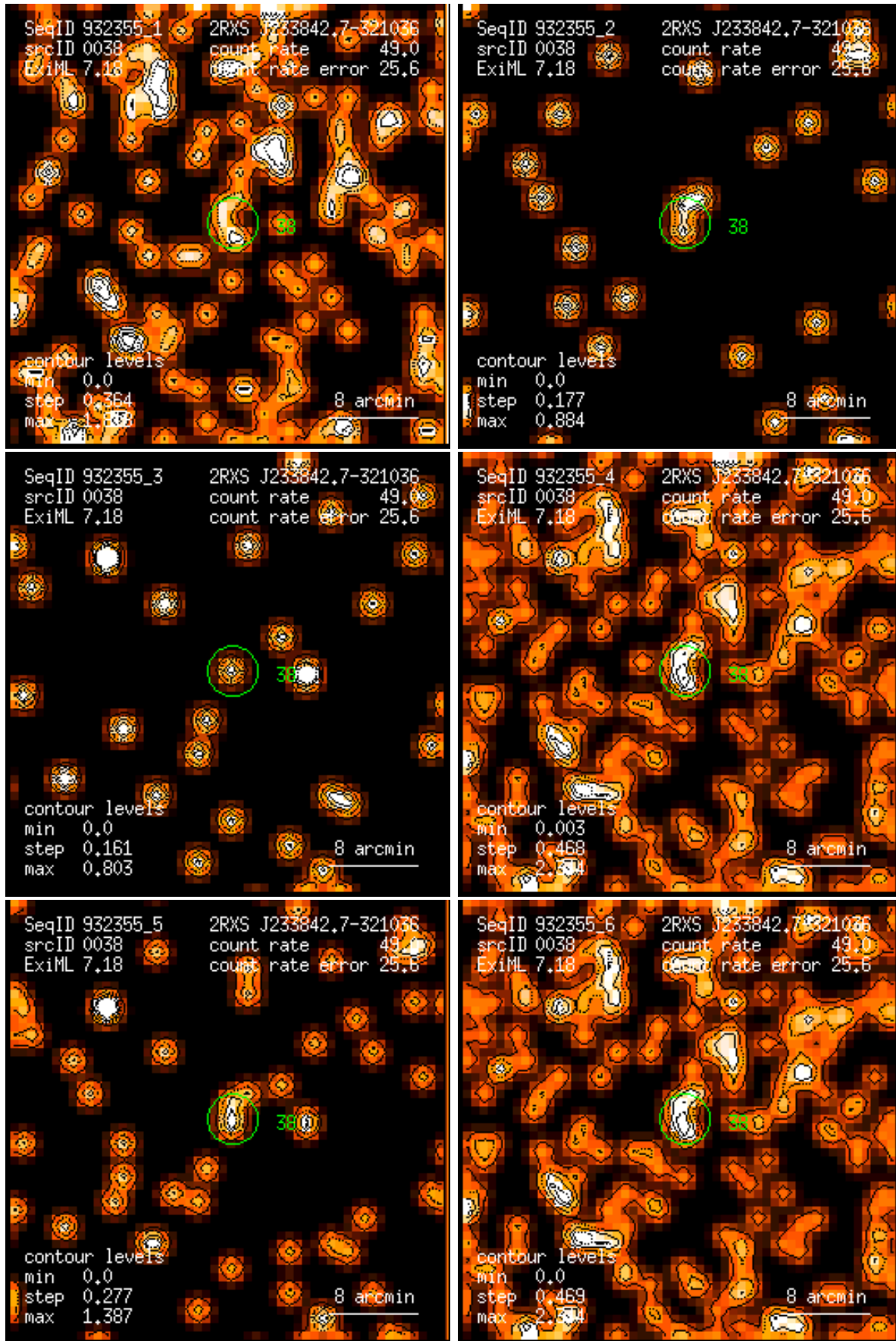
Figure 38: RASS 932355: detection 0038: band rate images, Gaussian filter: (1) PSPC channels 11 – 41, (2) 52 – 90, (3) 91 – 201, (4) 11 – 235, (5) 52 – 201, (6) 11 – 201. Broad band rates in counts/ks. Band rate contour levels in counts/ks/arcmin 2 .
