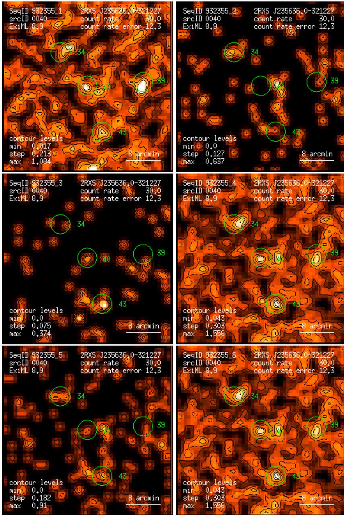
Figure 40: RASS 932355: detection 0040: band rate images, Gaussian filter: (1) PSPC channels 11 – 41, (2) 52 – 90, (3) 91 – 201, (4) 11 – 235, (5) 52 – 201, (6) 11 – 201. Broad band rates in counts/ks. Band rate contour levels in counts/ks/arcmin 2 .
