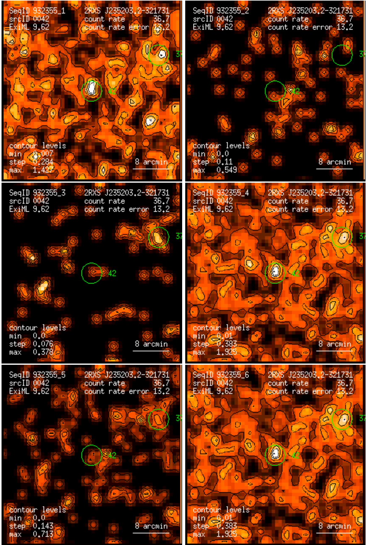
Figure 42: RASS 932355: detection 0042: band rate images, Gaussian filter: (1) PSPC channels 11 – 41, (2) 52 – 90, (3) 91 – 201, (4) 11 – 235, (5) 52 – 201, (6) 11 – 201. Broad band rates in counts/ks. Band rate contour levels in counts/ks/arcmin 2 .
