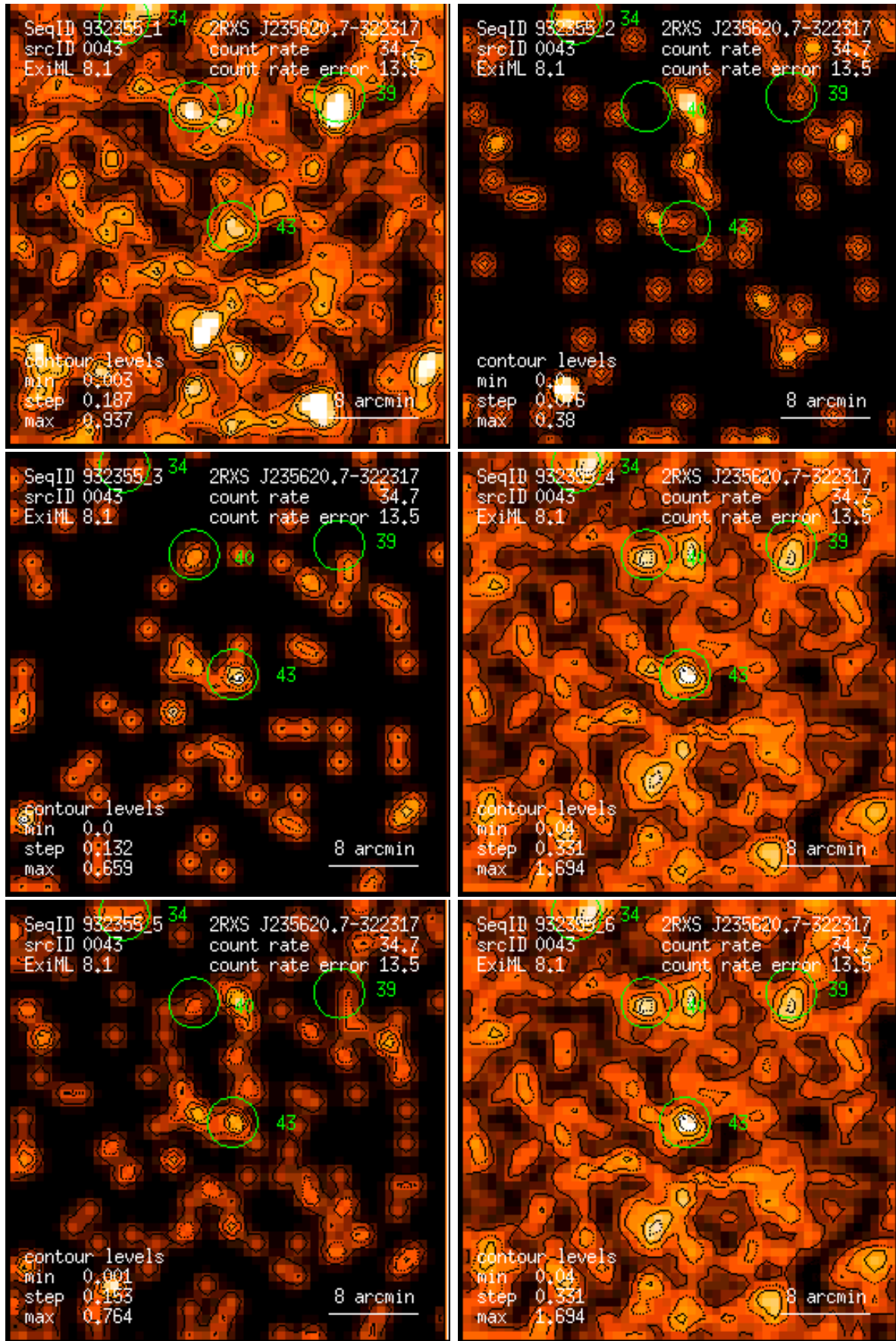
Figure 43: RASS 932355: detection 0043: band rate images, Gaussian filter: (1) PSPC channels 11 – 41, (2) 52 – 90, (3) 91 – 201, (4) 11 – 235, (5) 52 – 201, (6) 11 – 201. Broad band rates in counts/ks. Band rate contour levels in counts/ks/arcmin 2 .
