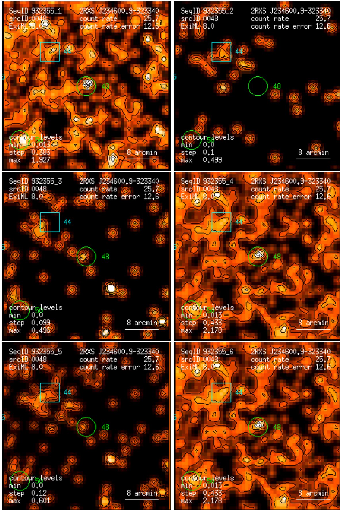
Figure 48: RASS 932355: detection 0048: band rate images, Gaussian filter: (1) PSPC channels 11 – 41, (2) 52 – 90, (3) 91 – 201, (4) 11 – 235, (5) 52 – 201, (6) 11 – 201. Broad band rates in counts/ks. Band rate contour levels in counts/ks/arcmin 2 .
