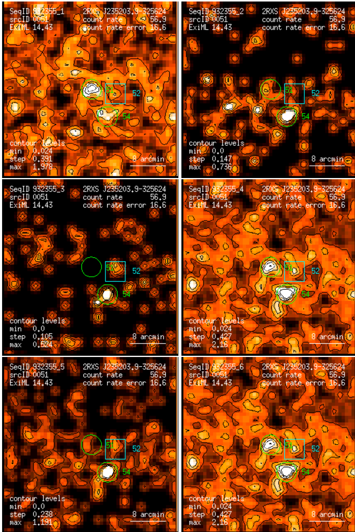
Figure 51: RASS 932355: detection 0051: band rate images, Gaussian filter: (1) PSPC channels 11 – 41, (2) 52 – 90, (3) 91 – 201, (4) 11 – 235, (5) 52 – 201, (6) 11 – 201. Broad band rates in counts/ks. Band rate contour levels in counts/ks/arcmin 2 .
