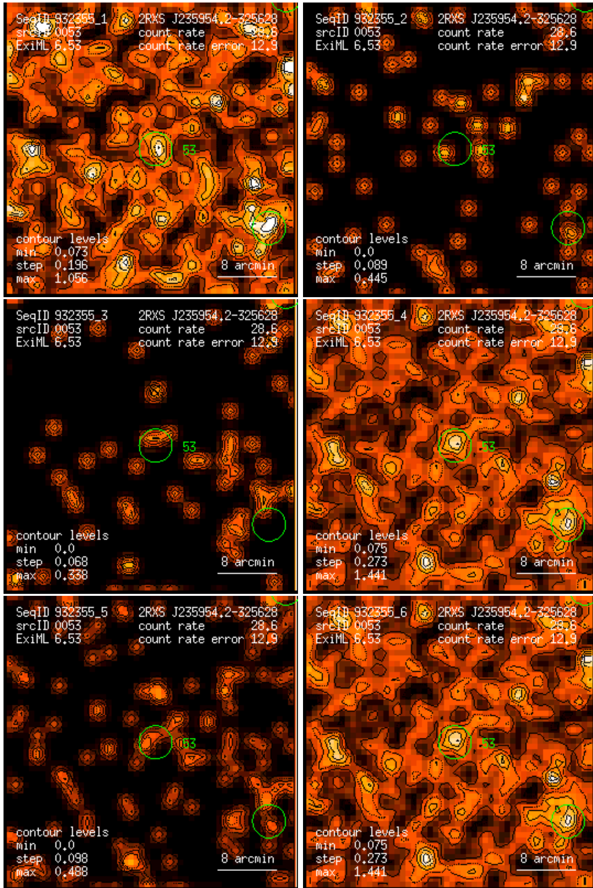
Figure 53: RASS 932355: detection 0053: band rate images, Gaussian filter: (1) PSPC channels 11 – 41, (2) 52 – 90, (3) 91 – 201, (4) 11 – 235, (5) 52 – 201, (6) 11 – 201. Broad band rates in counts/ks. Band rate contour levels in counts/ks/arcmin 2 .
