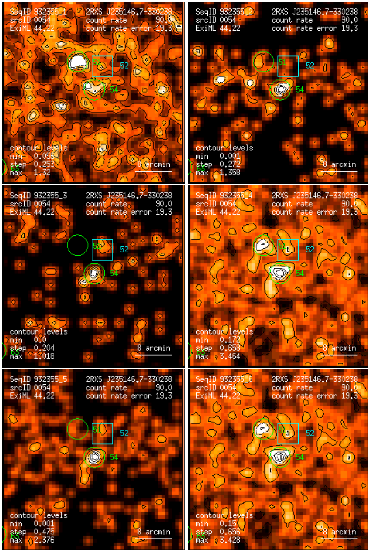
Figure 54: RASS 932355: detection 0054: band rate images, Gaussian filter: (1) PSPC channels 11 – 41, (2) 52 – 90, (3) 91 – 201, (4) 11 – 235, (5) 52 – 201, (6) 11 – 201. Broad band rates in counts/ks. Band rate contour levels in counts/ks/arcmin 2 .
