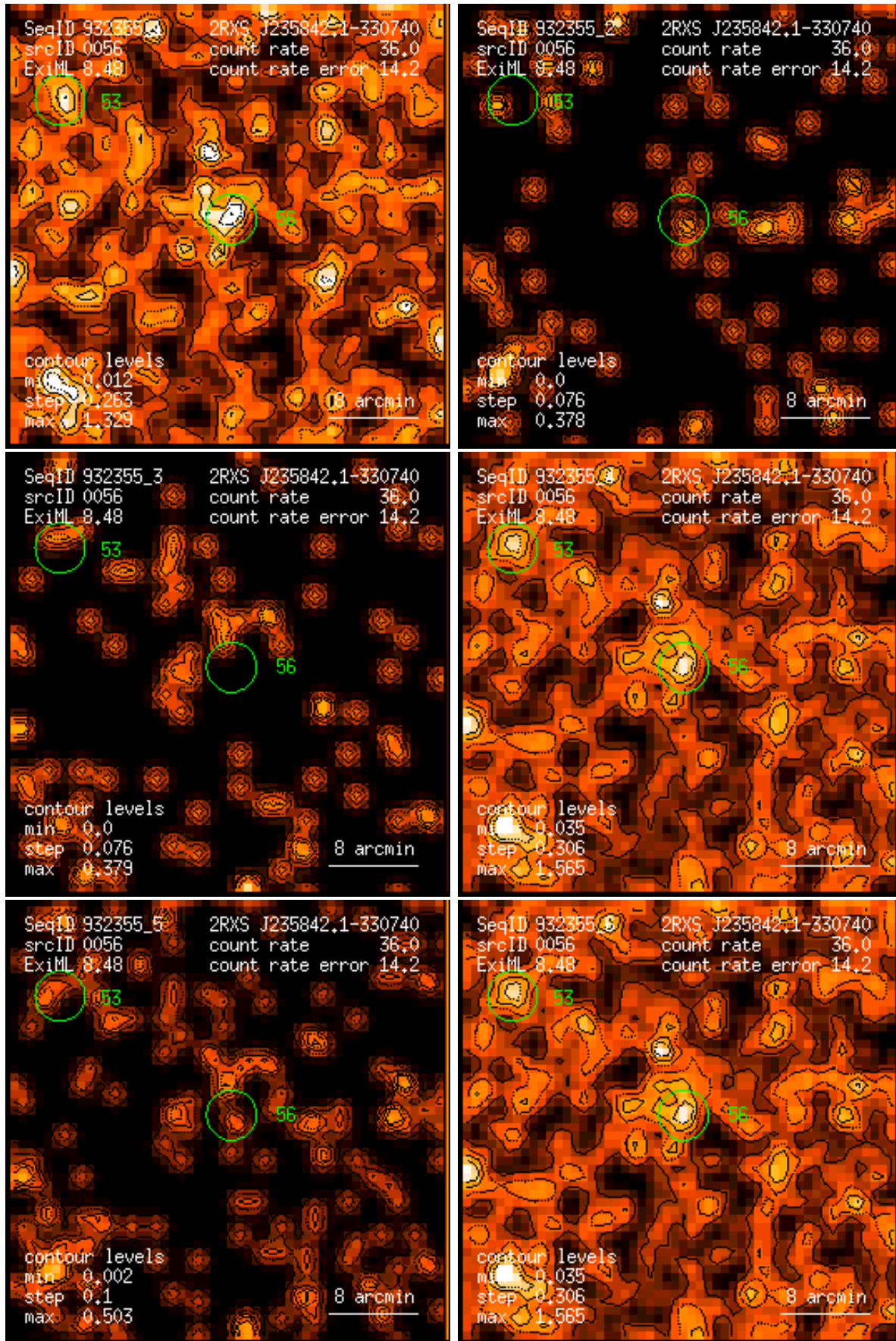
Figure 56: RASS 932355: detection 0056: band rate images, Gaussian filter: (1) PSPC channels 11 – 41, (2) 52 – 90, (3) 91 – 201, (4) 11 – 235, (5) 52 – 201, (6) 11 – 201. Broad band rates in counts/ks. Band rate contour levels in counts/ks/arcmin 2 .
