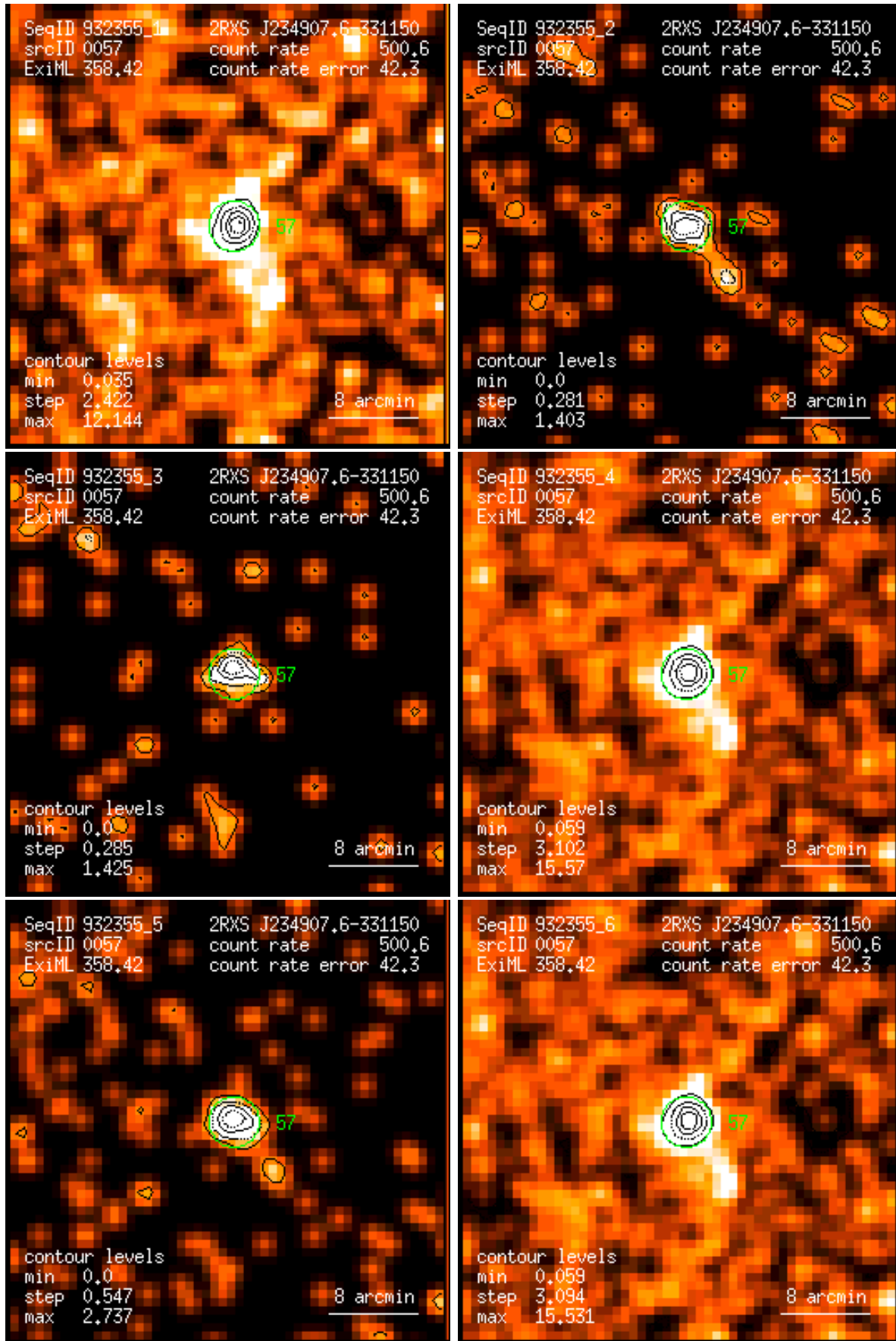
Figure 57: RASS 932355: detection 0057: band rate images, Gaussian filter: (1) PSPC channels 11 – 41, (2) 52 – 90, (3) 91 – 201, (4) 11 – 235, (5) 52 – 201, (6) 11 – 201. Broad band rates in counts/ks. Band rate contour levels in counts/ks/arcmin 2 .
