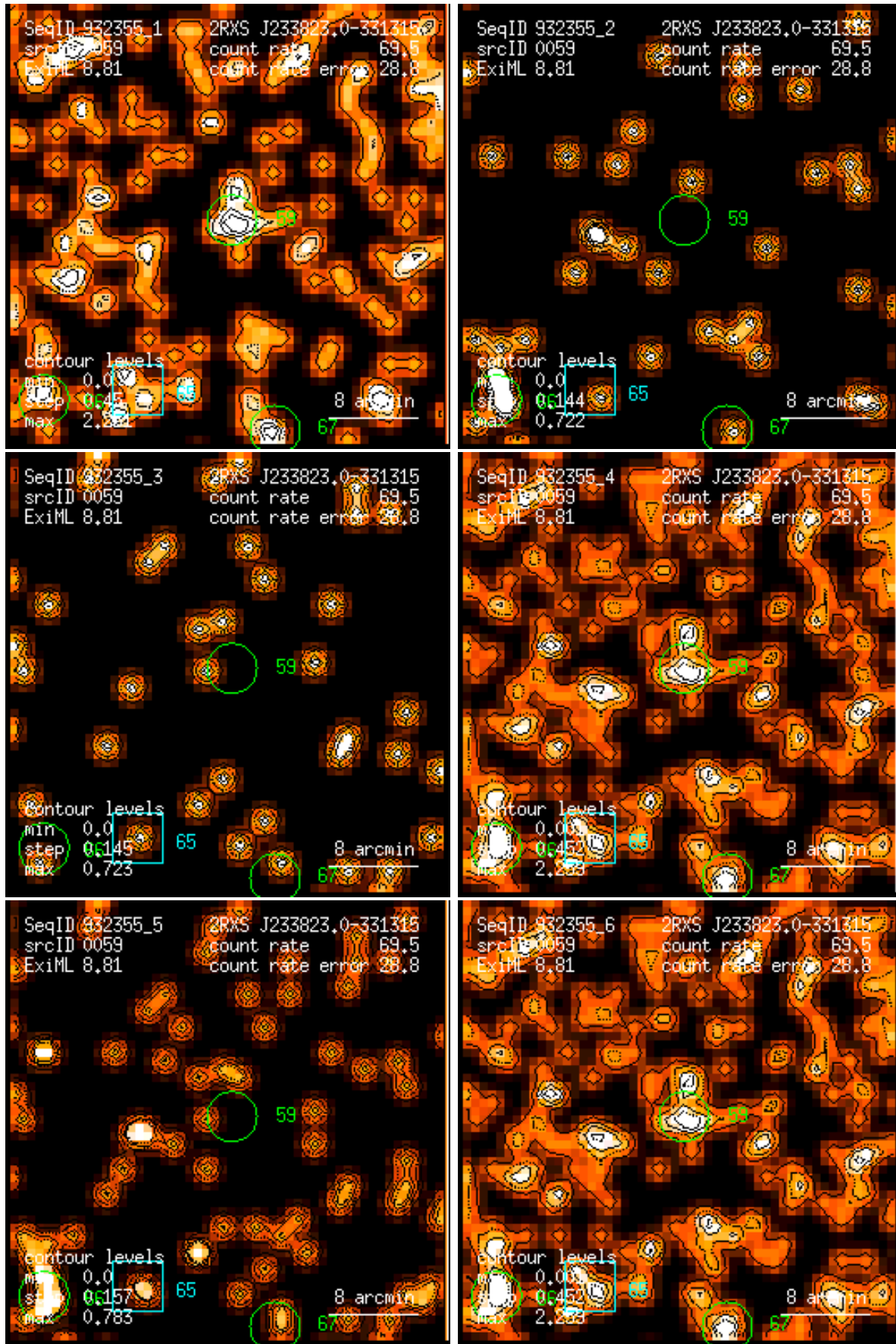
Figure 59: RASS 932355: detection 0059: band rate images, Gaussian filter: (1) PSPC channels 11 – 41, (2) 52 – 90, (3) 91 – 201, (4) 11 – 235, (5) 52 – 201, (6) 11 – 201. Broad band rates in counts/ks. Band rate contour levels in counts/ks/arcmin 2 .
