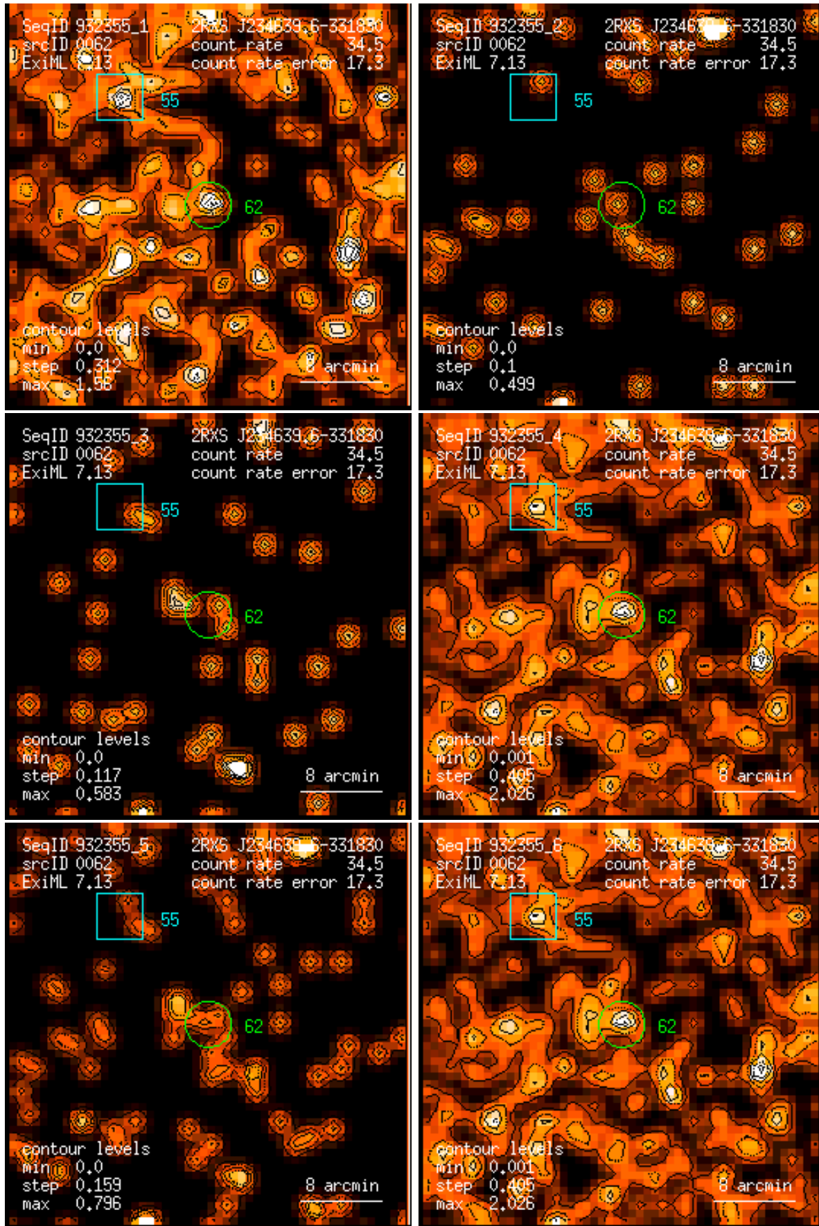
Figure 62: RASS 932355: detection 0062: band rate images, Gaussian filter: (1) PSPC channels 11 – 41, (2) 52 – 90, (3) 91 – 201, (4) 11 – 235, (5) 52 – 201, (6) 11 – 201. Broad band rates in counts/ks. Band rate contour levels in counts/ks/arcmin 2 .
