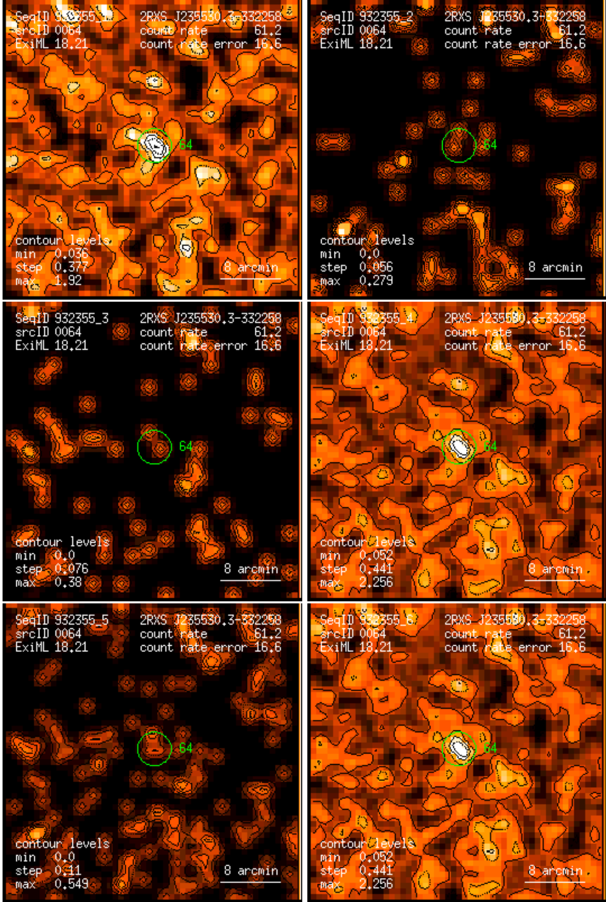
Figure 64: RASS 932355: detection 0064: band rate images, Gaussian filter: (1) PSPC channels 11 – 41, (2) 52 – 90, (3) 91 – 201, (4) 11 – 235, (5) 52 – 201, (6) 11 – 201. Broad band rates in counts/ks. Band rate contour levels in counts/ks/arcmin 2 .
