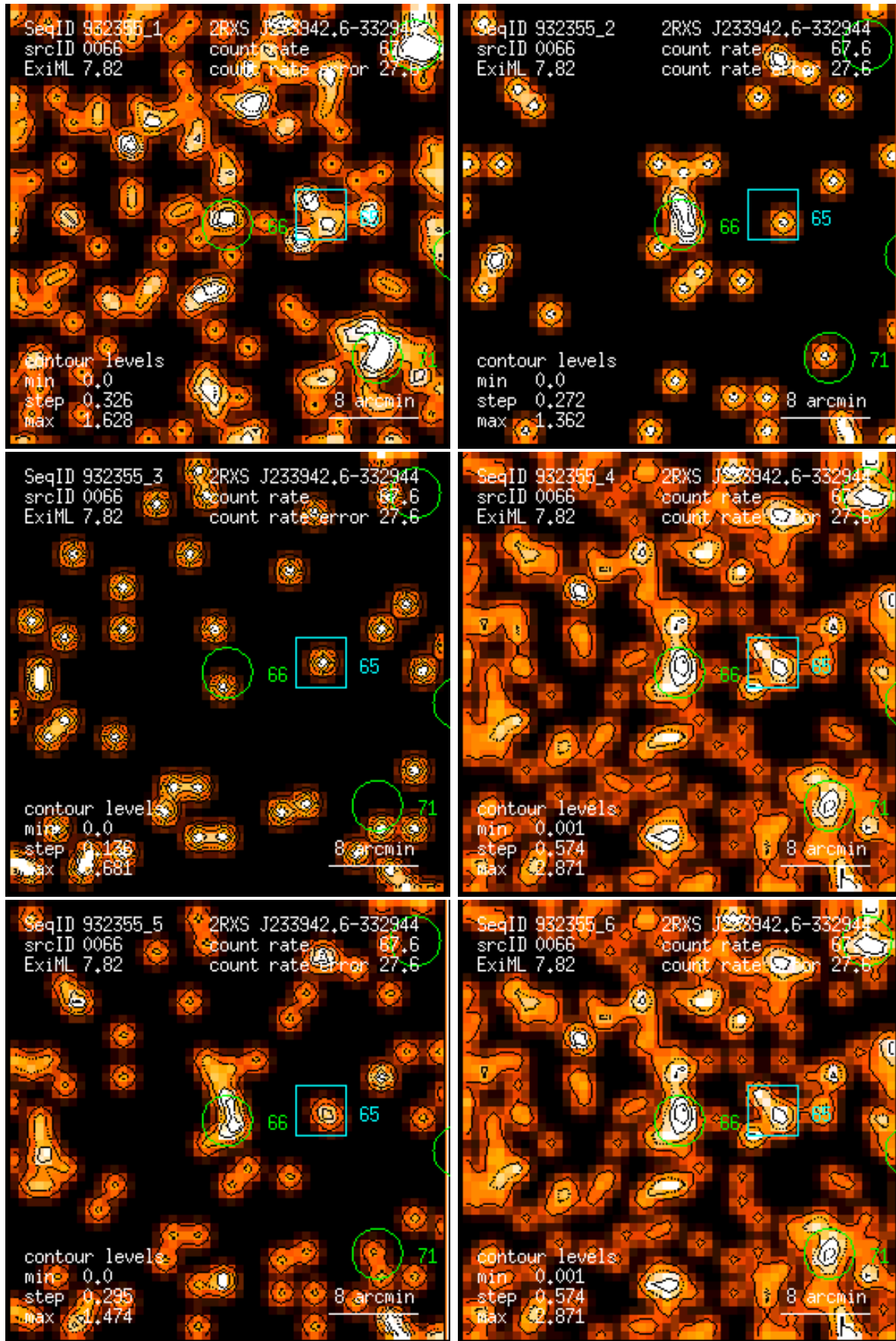
Figure 66: RASS 932355: detection 0066: band rate images, Gaussian filter: (1) PSPC channels 11 – 41, (2) 52 – 90, (3) 91 – 201, (4) 11 – 235, (5) 52 – 201, (6) 11 – 201. Broad band rates in counts/ks. Band rate contour levels in counts/ks/arcmin 2 .
