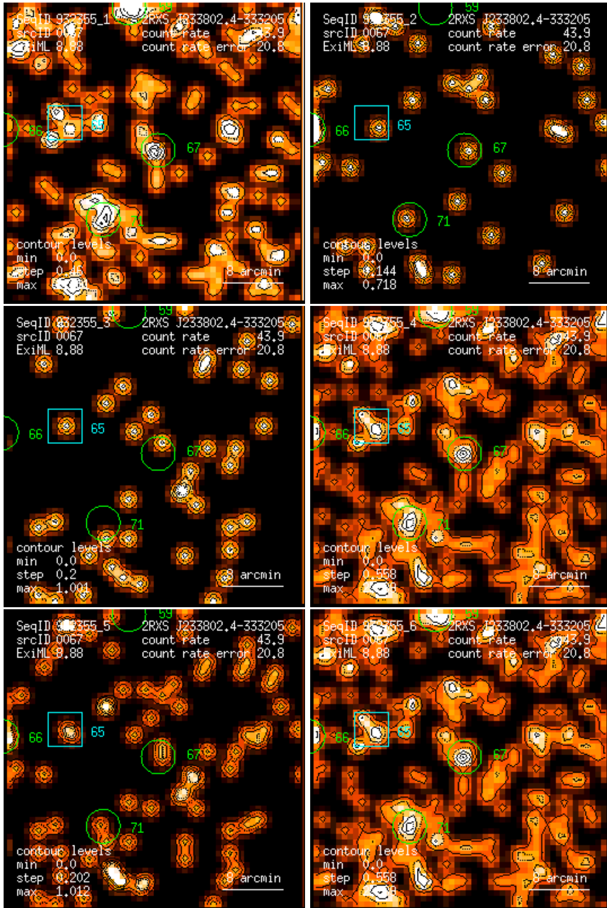
Figure 67: RASS 932355: detection 0067: band rate images, Gaussian filter: (1) PSPC channels 11 – 41, (2) 52 – 90, (3) 91 – 201, (4) 11 – 235, (5) 52 – 201, (6) 11 – 201. Broad band rates in counts/ks. Band rate contour levels in counts/ks/arcmin 2 .
