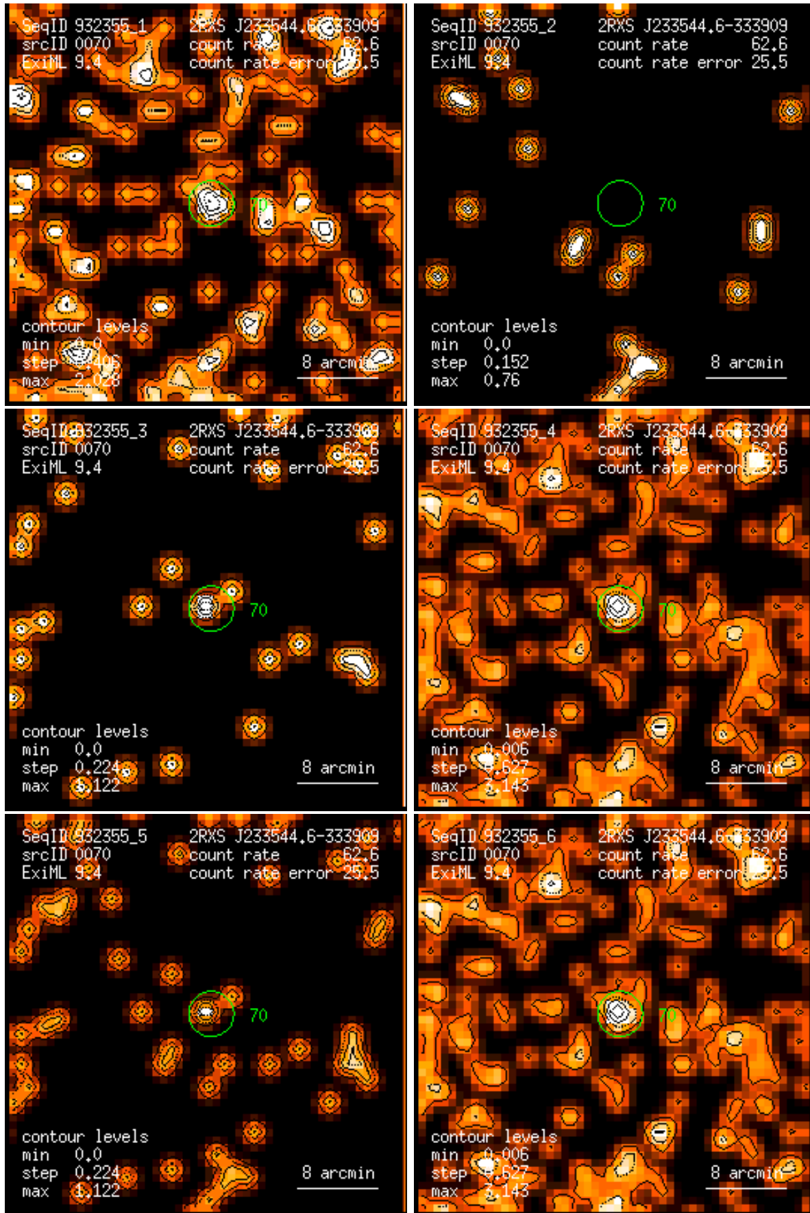
Figure 70: RASS 932355: detection 0070: band rate images, Gaussian filter: (1) PSPC channels 11 – 41, (2) 52 – 90, (3) 91 – 201, (4) 11 – 235, (5) 52 – 201, (6) 11 – 201. Broad band rates in counts/ks. Band rate contour levels in counts/ks/arcmin 2 .
