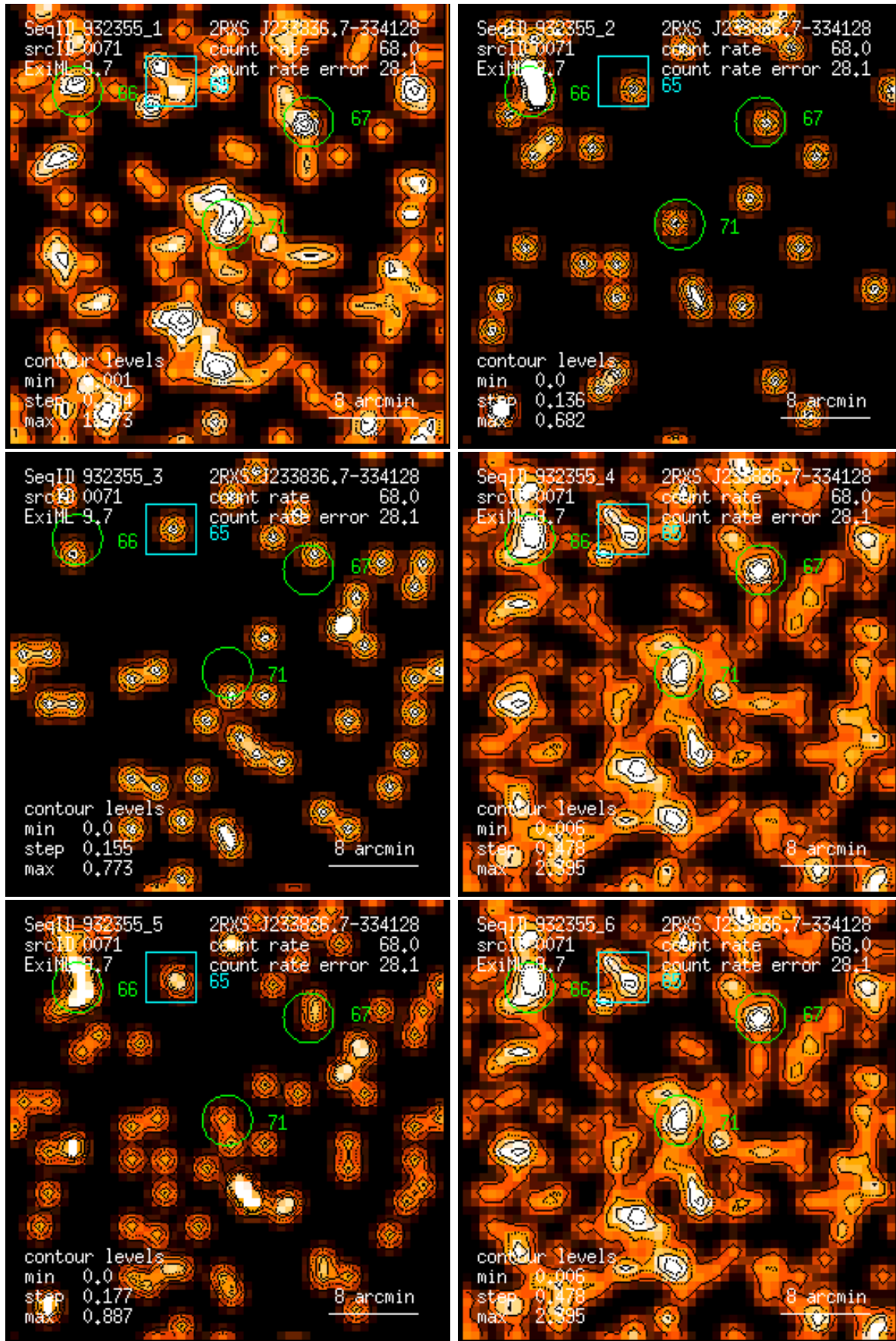
Figure 71: RASS 932355: detection 0071: band rate images, Gaussian filter: (1) PSPC channels 11 – 41, (2) 52 – 90, (3) 91 – 201, (4) 11 – 235, (5) 52 – 201, (6) 11 – 201. Broad band rates in counts/ks. Band rate contour levels in counts/ks/arcmin 2 .
