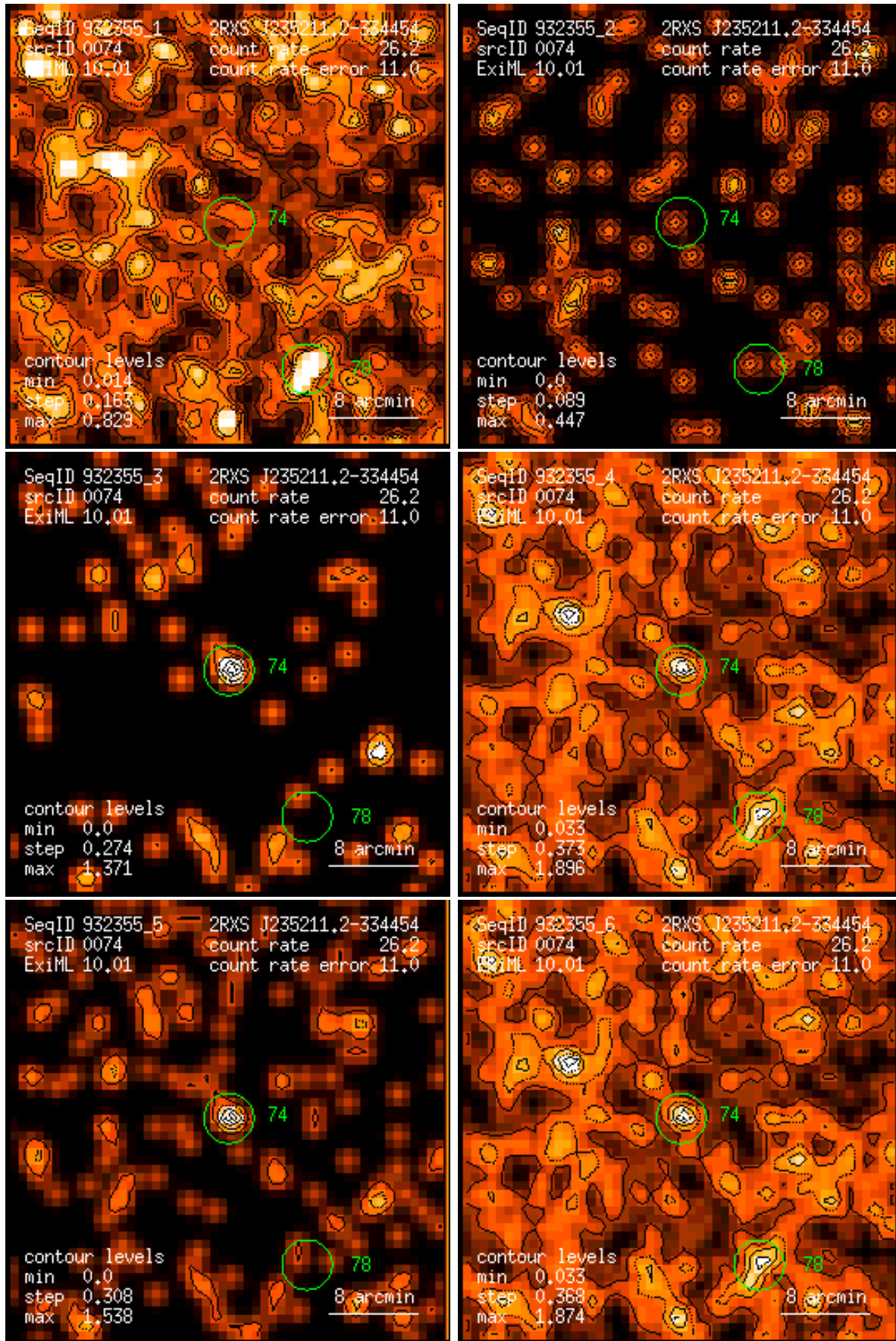
Figure 74: RASS 932355: detection 0074: band rate images, Gaussian filter: (1) PSPC channels 11 – 41, (2) 52 – 90, (3) 91 – 201, (4) 11 – 235, (5) 52 – 201, (6) 11 – 201. Broad band rates in counts/ks. Band rate contour levels in counts/ks/arcmin 2 .
