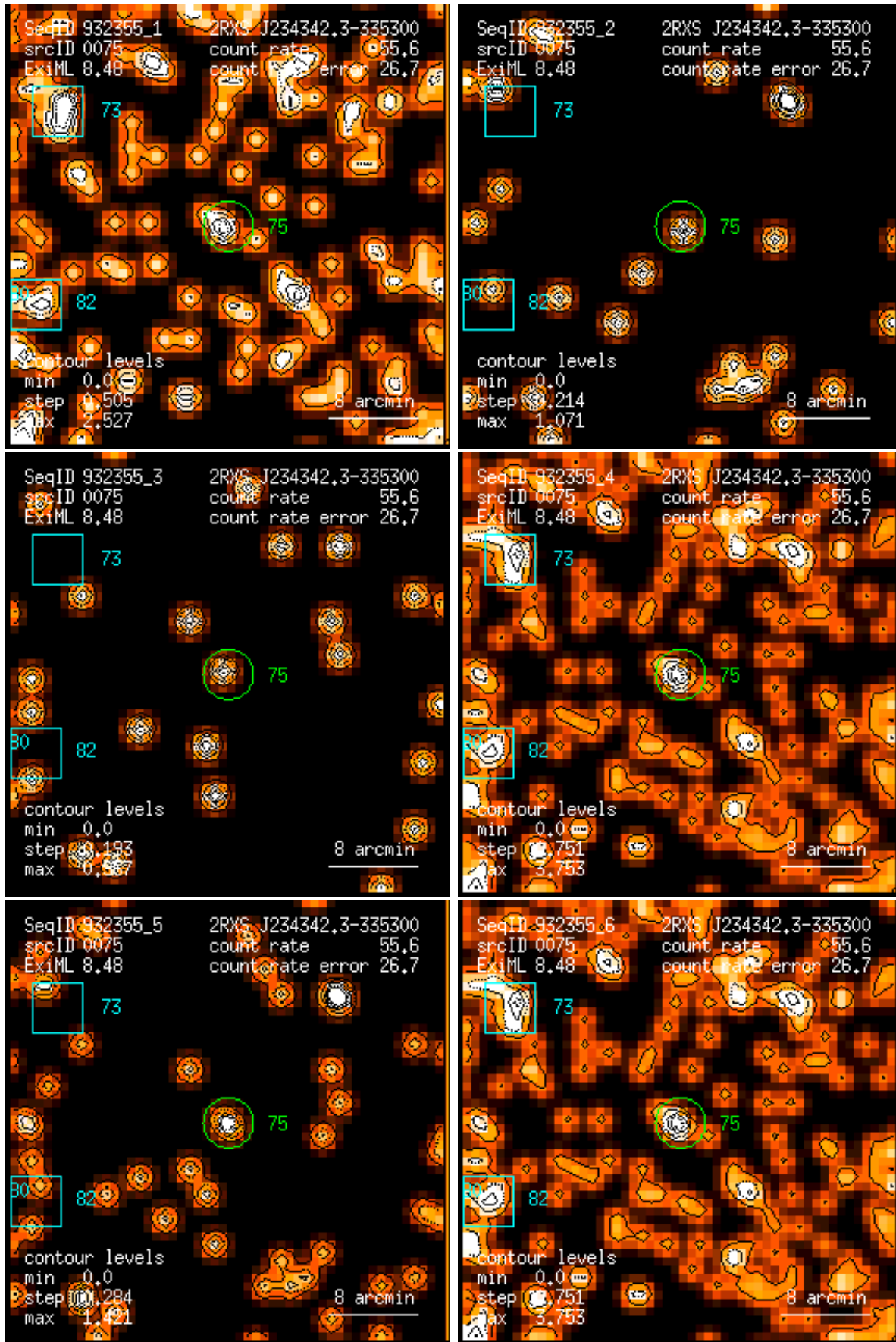
Figure 75: RASS 932355: detection 0075: band rate images, Gaussian filter: (1) PSPC channels 11 – 41, (2) 52 – 90, (3) 91 – 201, (4) 11 – 235, (5) 52 – 201, (6) 11 – 201. Broad band rates in counts/ks. Band rate contour levels in counts/ks/arcmin 2 .
