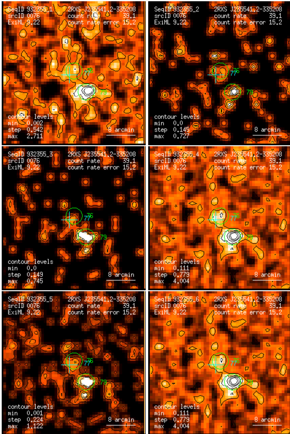
Figure 76: RASS 932355: detection 0076: band rate images, Gaussian filter: (1) PSPC channels 11 – 41, (2) 52 – 90, (3) 91 – 201, (4) 11 – 235, (5) 52 – 201, (6) 11 – 201. Broad band rates in counts/ks. Band rate contour levels in counts/ks/arcmin 2 .
