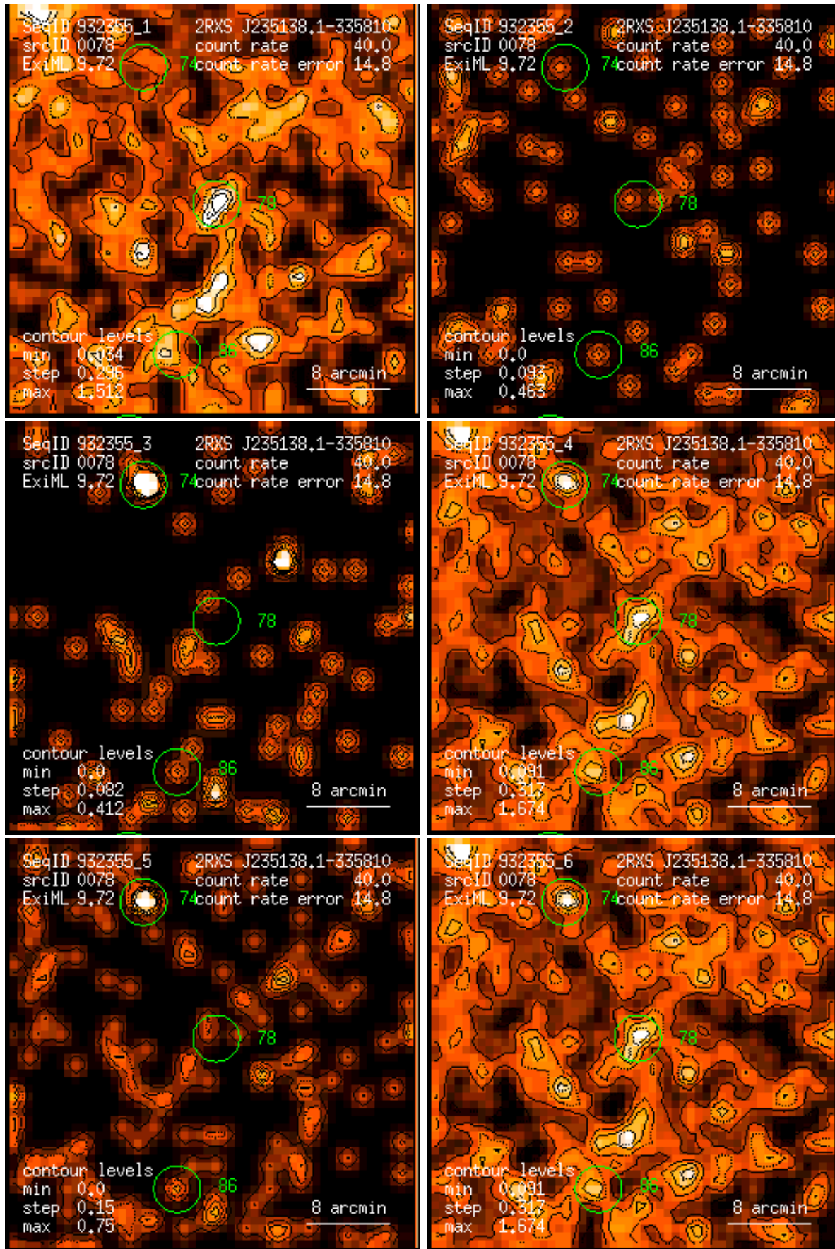
Figure 78: RASS 932355: detection 0078: band rate images, Gaussian filter: (1) PSPC channels 11 – 41, (2) 52 – 90, (3) 91 – 201, (4) 11 – 235, (5) 52 – 201, (6) 11 – 201. Broad band rates in counts/ks. Band rate contour levels in counts/ks/arcmin 2 .
